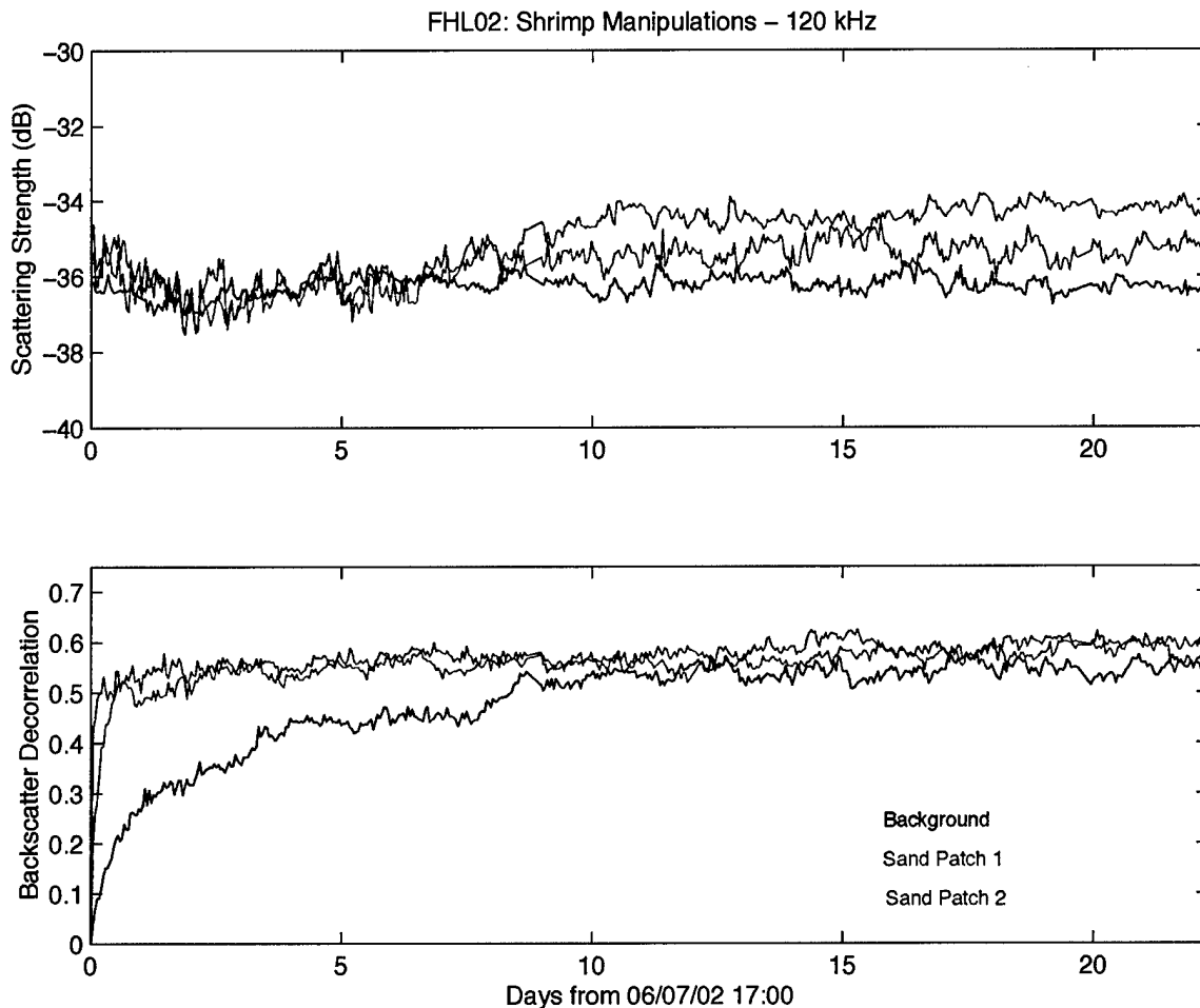
Figure 3. Backscatter and backscatter decorrelation from the two patches over time after the introduction of burrowing, thalassinid shrimp. Both are enhanced by the manipulation, but the backscatter increase lasts more than three weeks whereas the decorrelation effect is largely limited to the first week.
