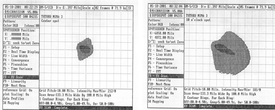
Figure A-3. Measured spot contours for the second sample monitor at screen center and the upper left corner at 168fL in 1600 x 1200 x 72Hz.
