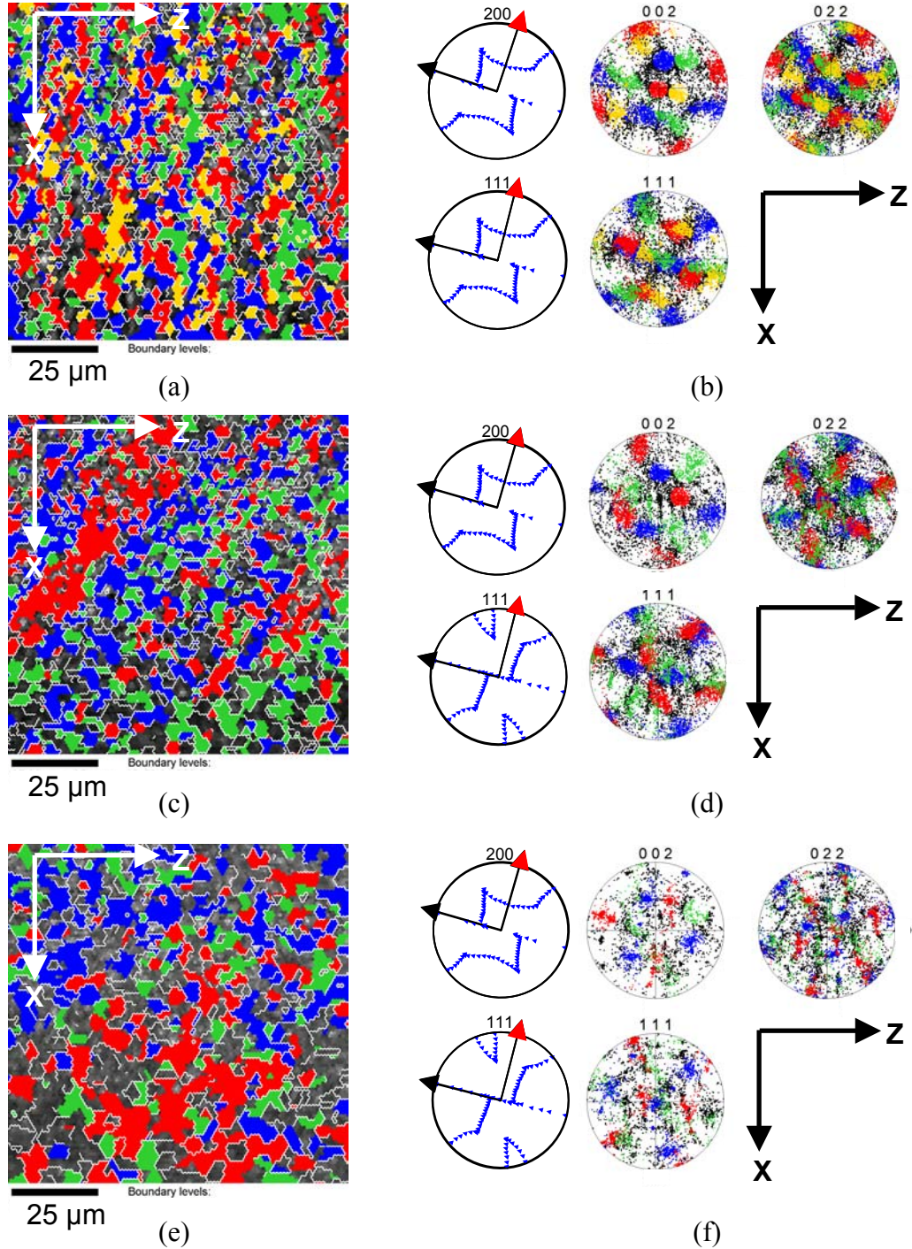
Figure 7.15. OIM IQ only maps with regions corresponding to the associated discrete pole figures highlighted along with boundaries in excess of 40^\circ (in white) from regions 100\mu\text{m}^2 of Al-3%Mg-0.2%Sc after eight ECAP passes and a 400^\circ\text{C} anneal to simulate times encountered during superplastic deformation via route A in (a) and (b), route B C in (c) and (d) and route C in (e) and (f). The shear texture intensities are as follows: in route A, A type 4.5x random, B type 8.5x random; route B C , A type 1.5x random, B type 3x random; and route C, A type 13x random, B type equal to random.
