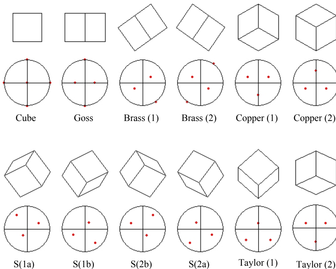
Figure 2.12. Schematic representations of a unit cube and the associated (200) pole figure, using the convention of RD being the vertical axis and TD the horizontal, for some common single orientation variants seen during rolling of fcc materials.
