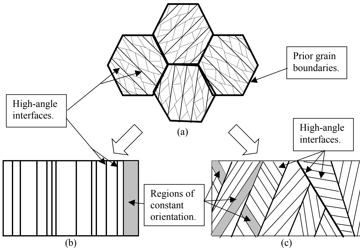
Figure 9.1. Schematic representation of deformation banding occurring during deformation. In (a), the prior grain boundaries are evident along with the high-angle interfaces separating the bands and the low-angle boundaries within each band, all formed during the early stages of processing. In (b), the band alignment in one direction results from each band orienting to deform with a minimum of active slip systems. The prior grain boundaries are indistinguishable from the high-angle interfaces formed during deformation. Also present, though not shown schematically, would be the presence of low-angle boundaries within each band. In (c), varying strain paths cause local variations of stress and strain resulting in the formation of high-angle interfaces within each band. Also implied are the low-angle boundaries within each band but not depicted here.
