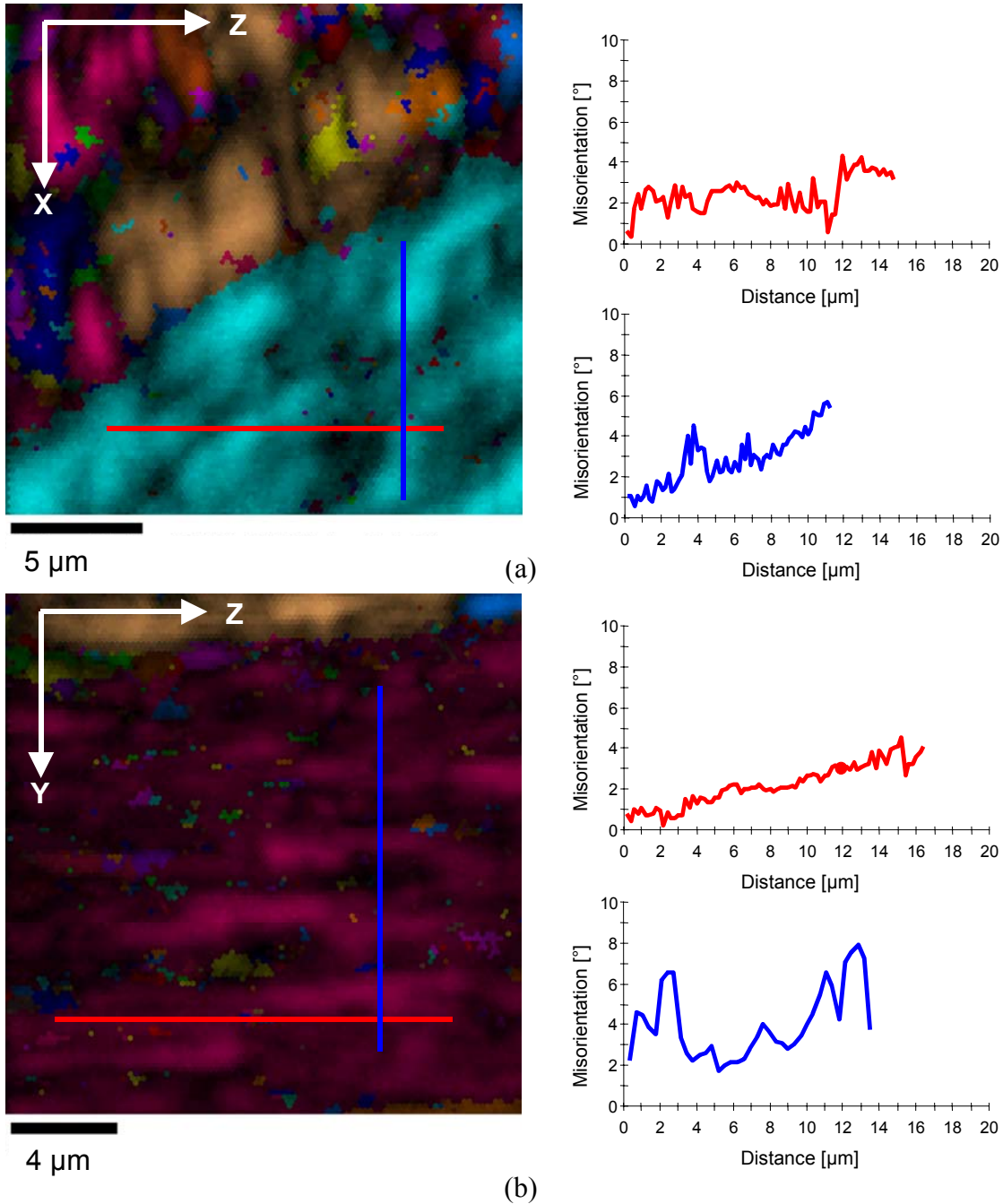
(b) Figure 7.6. OIM data from pure aluminum after one ECAP pass. A representative example of y plane data in (a) showing a unique grain color map with IQ superimposed, the locations of the z and x linear profiles, and the associated misorientation profiles in red and blue respectively. In (b), a representative example of x plane data again showing a unique grain color map with IQ superimposed, the locations of the z and y linear profiles, and the associated misorientation profiles in red and blue respectively.
