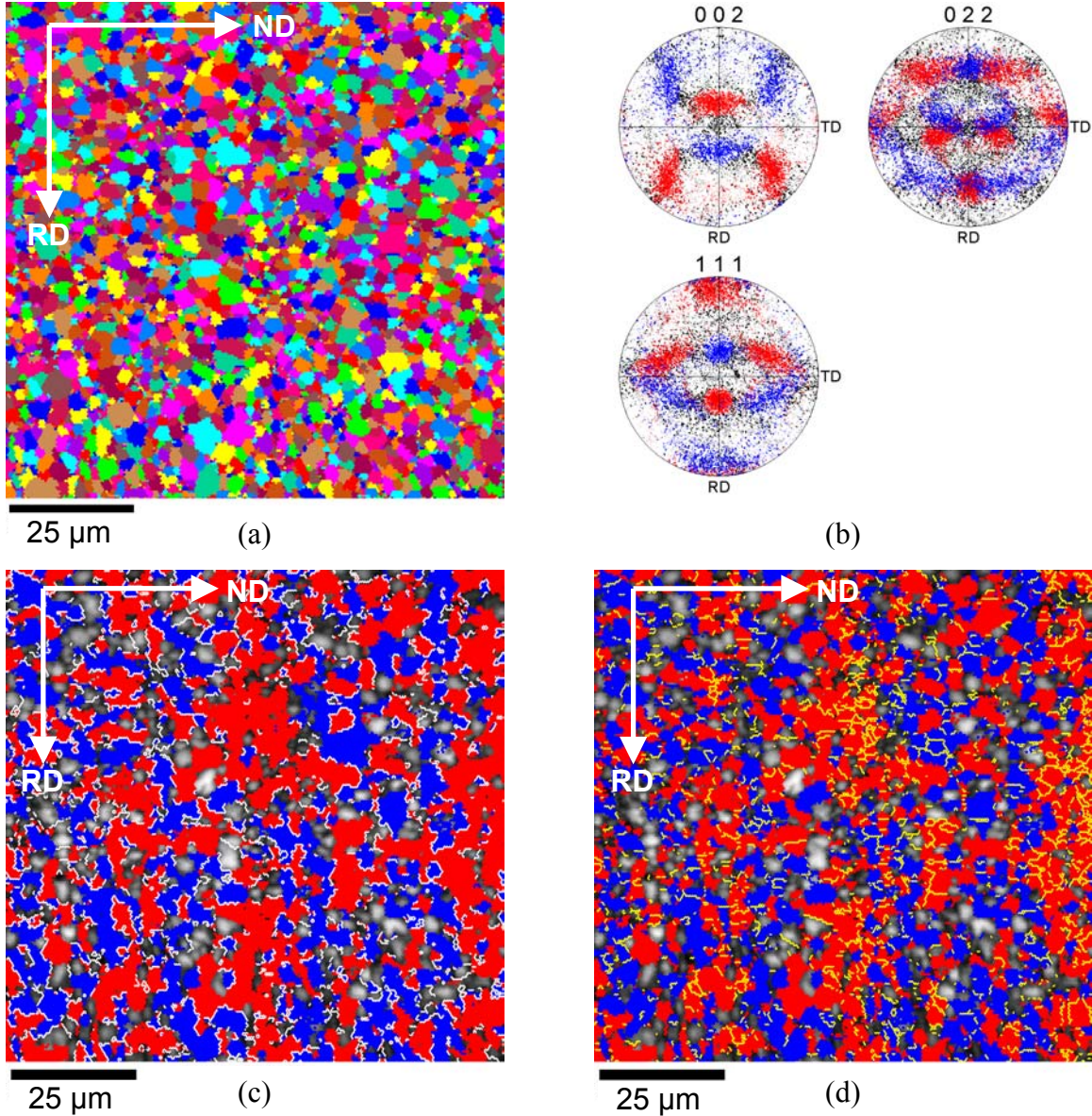
Figure 6.2. OIM data for Al-5%Ca-5%Zn after annealing at 520°C for 15min.: (a) an OIM unique grain color map for (sub)grains disoriented more than 2^\circ ; (b), discrete pole figures in which the two variants of the C texture component have been highlighted in either red or blue; (c) and (d) IQ only maps plotted with the positions of the high-angle ( 50^\circ < \theta < 62.8^\circ ) and low-angle ( 2^\circ < \theta < 15^\circ ) boundaries highlighted in white and yellow respectively along with the locations of the two C texture components highlighted in red and blue corresponding to (b).
