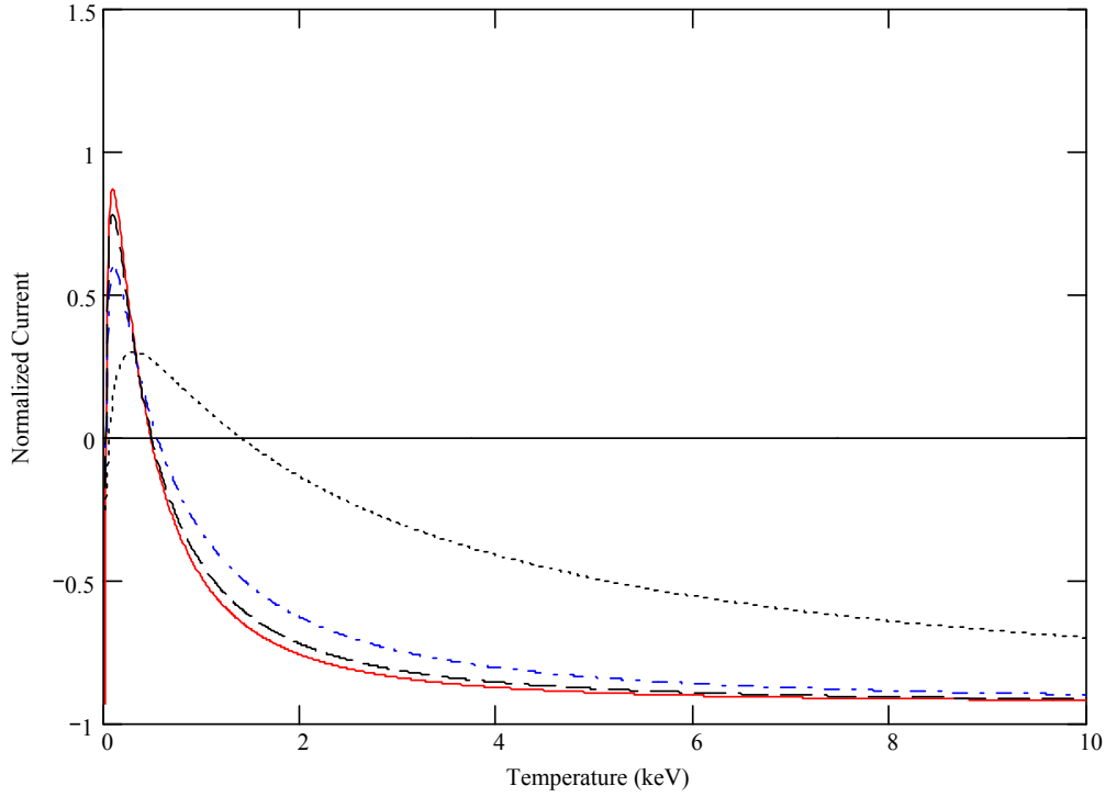
Figure 7 Normalized Current I/I_0 vs. Electron Temperature for kapton. Curves are the kappa Current Balance Equation with \kappa = 1.6 (dot), \kappa = 2.5 (dash-dot), \kappa = 5.5 (dash), and the Maxwellian Current Balance Equation (solid).
