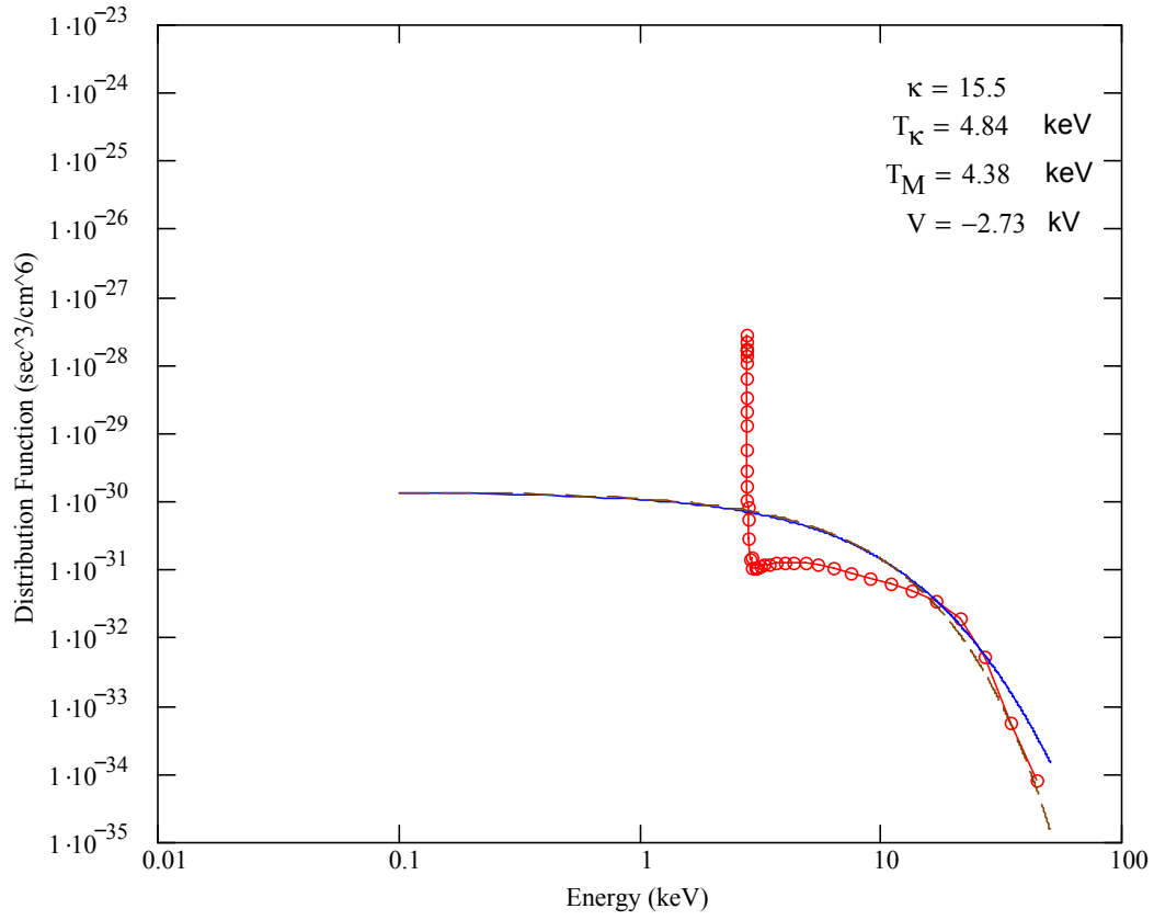
Figure 29 Electron Distribution Function vs. Energy at 19.18 UT (23.84 LT) on 14 March 1999 from LANL 1997A Data. Displayed are the Data Derived (circles), the kappa (solid), and the Maxwellian (dash) Distribution Functions. (Data Courtesy of Michelle F. Thomsen, Los Alamos National Laboratory.)
