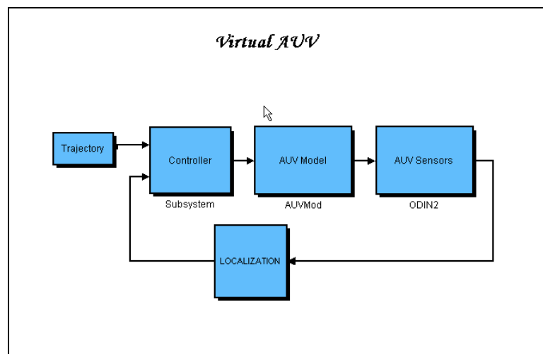
Figure LN-6 – SAUVIM simulation of the Navigation system using Simulink and OpenGL.
