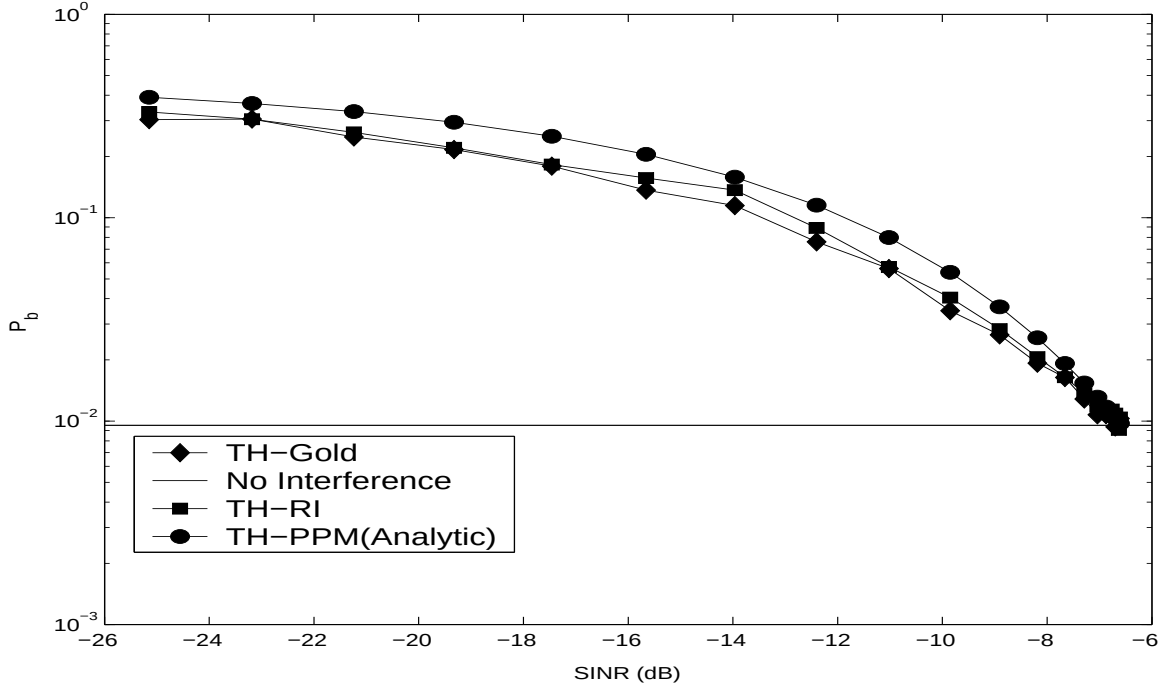
Figure 4.23 TH-PPM Centered DSSS Interference Results for E_b/N_o = 7.5 dB
