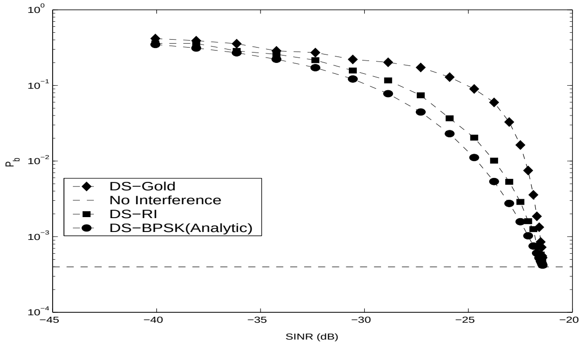
Figure 4.24 DS-BPSK Centered DSSS Interference Results for E_b/N_o = 7.5 dB
