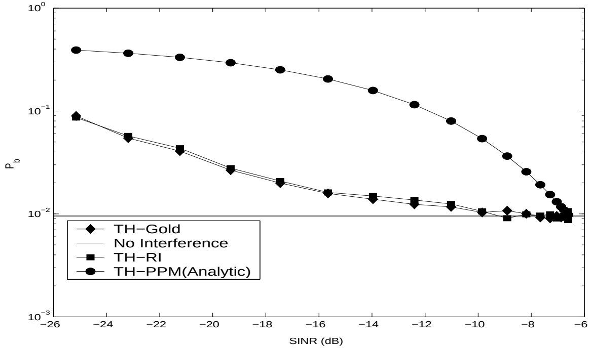
Figure 4.21 TH-PPM Offset DSSS Interference Results for E_b/N_o = 7.5 dB
