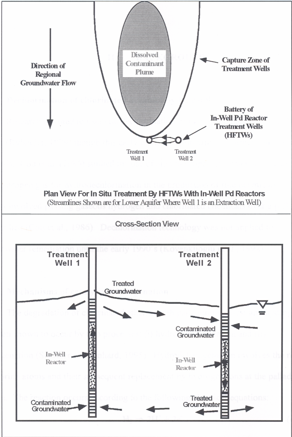
Figure 1.1 Horizontal Flow Treatment Well System (from Stoppel, 2001)
