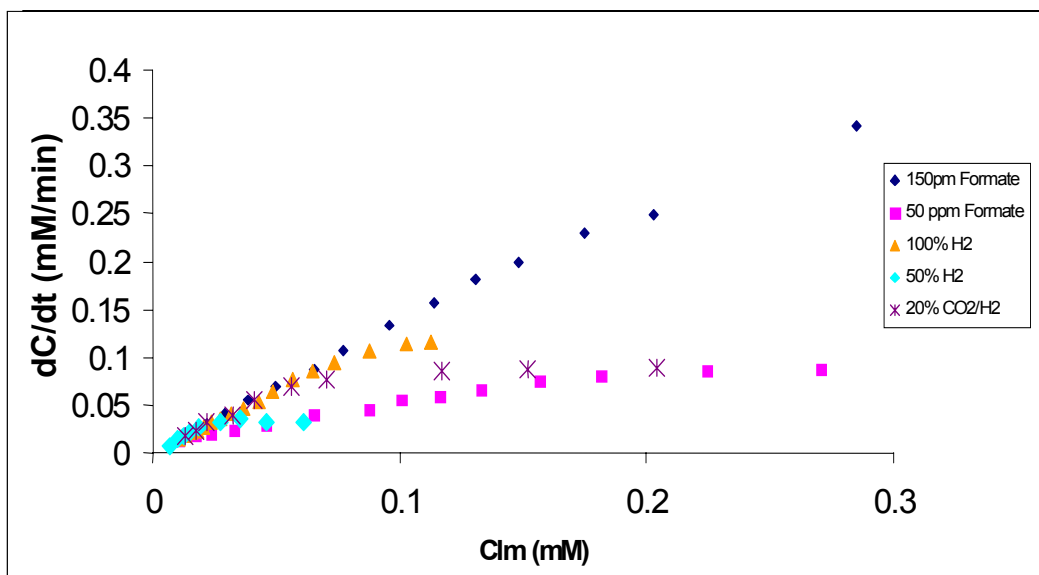
Figure 4.10 Comparison of the Effect of Reductant Type and Concentration on 2-NT Degradation Rates Fraction of 2-NT removed for the three reductants was also plotted (see Figure 4.11). As can be seen, the fraction of 2-NT removal when 150 ppm formate is used as a reductant remains at a constant level and does not decrease with log-mean 2-NT concentration as the fraction removal does for the other three reductants.
