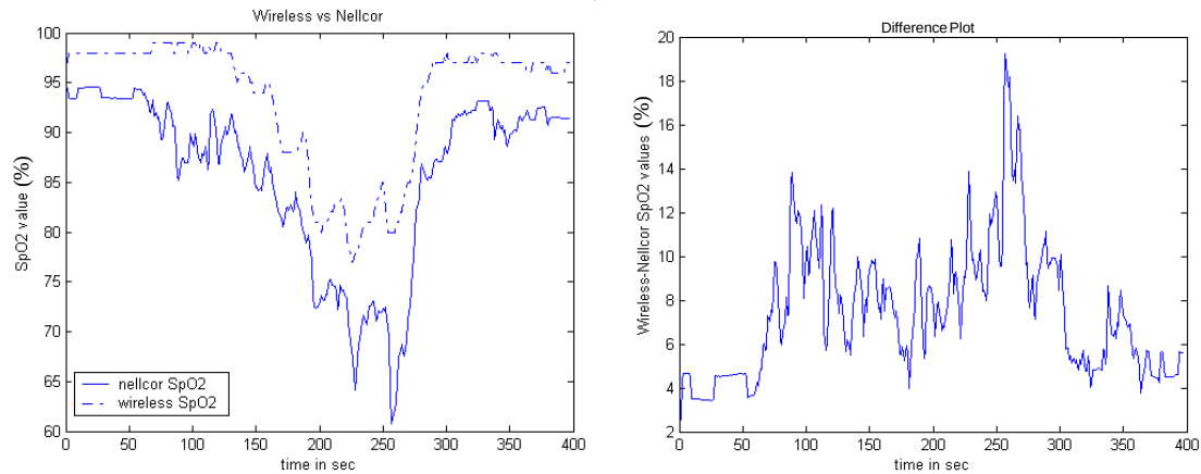
Figure 36. Wireless vs Nellcor and error plots for Test Case 8
