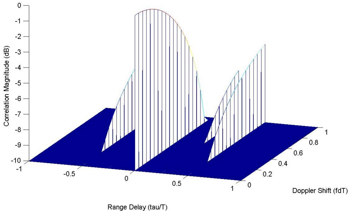
Figure 3.2: Ambiguity diagram for the Welty coded waveform
