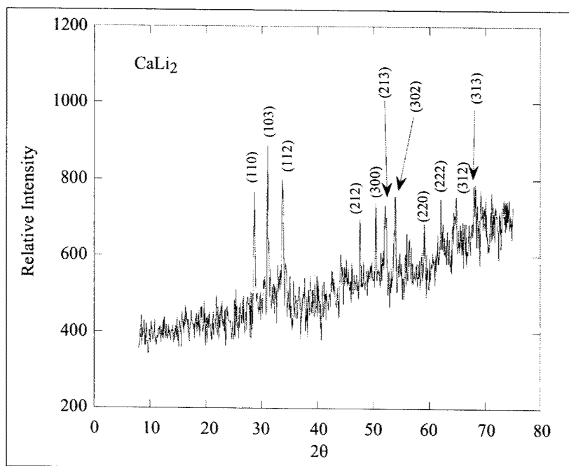
Figure 1. X-ray diffraction pattern of the CaLi 2 powders.
