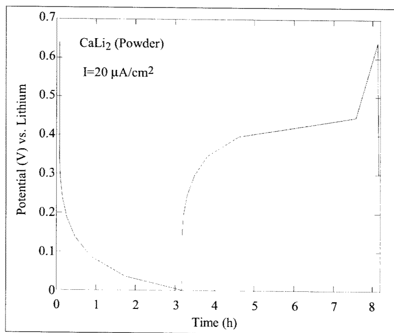
Figure 2. Charge-discharge curve of the CaLi 2 powders at room temperature.
