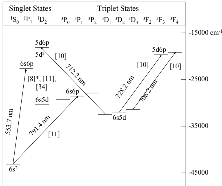
Figure 3-5. Lower electronic energy states of atomic barium. Transitions studied previously are referenced. The asterisk indicates theoretical work.
