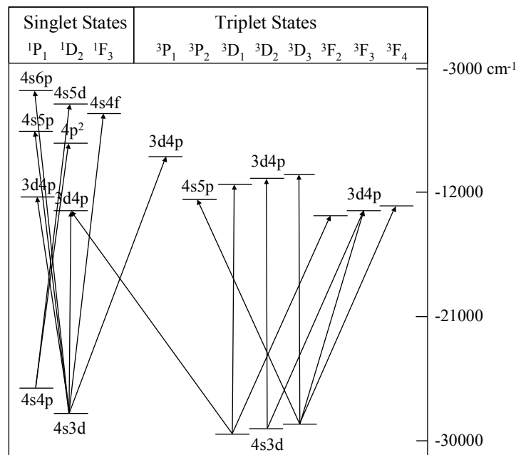
Figure 3-3. Mid-level electronic energy states of atomic calcium. Transitions studied by Smith and Raggett [47] are noted.
