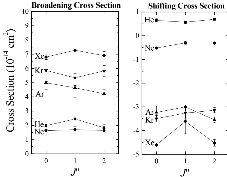
Figure 4-10. Line broadening and shifting cross sections of the atomic strontium 5s5p\ ^3P_{0,1,2} \rightarrow 5s6s\ ^3S_1 transitions around 14534 \text{ cm}^{-1} perturbed by helium, neon, argon, krypton, and xenon as a function of the total angular momentum quantum number J'' of the initial state. These cross sections are computed from the line broadening and shifting rates presented in Table 4-4 using Equations 4-15 and 4-16.
