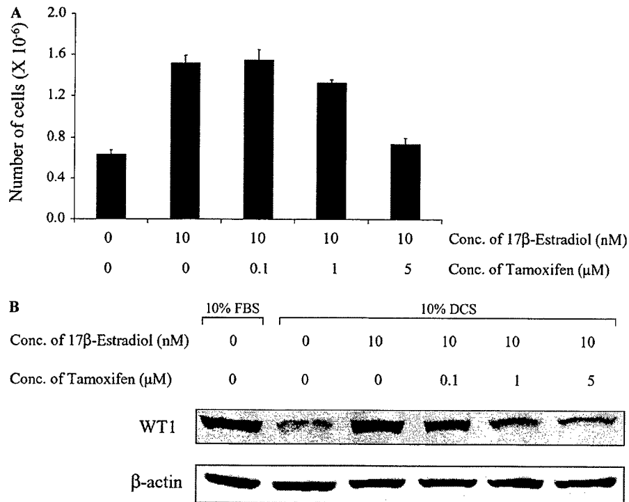
Fig. 2. 17 \beta -Estradiol increased WT1 protein expression but tamoxifen decreased WT1 expression in MCF-7 cells. (A) MCF-7 cells were seeded in triplicate (at 1.5 \times 10^5 per well) in six-well plates in DMEM/F12 medium supplemented with 10% FBS and incubated for 24 h. The medium was then changed to phenol red-free DMEM/F12 medium supplemented with 10% DCS and 10 nM 17 \beta -estradiol. Various concentrations of tamoxifen (0, 0.1, 1, or 5 \mu M) were added to cells and the cells were then incubated for an additional 72 h. Cells were harvested and counted by trypan blue dye exclusion. The numbers of MCF-7 cells are expressed as means \pm SD. (B) Fifty \mu g proteins were used to analyze WT1 expression by Western blot analysis. Data were quantified by scanning densitometry and WT1 levels were normalized to \beta -actin levels.
