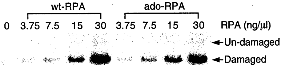
Figure 4. RPA- dependent nucleotide excision repair (NER)
