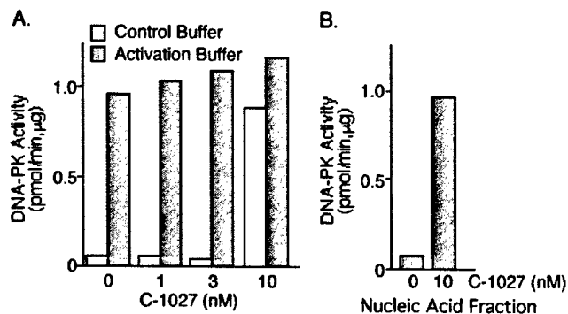
FIGURE 4: Treatment of cells with high levels of C-1027 generates DNA fragments sufficient to induce DNA-PK activity. (A) 40 \mu\text{g} of total protein from hypotonic extracts of 293 cells treated with the indicated concentrations of C-1027 for 2 h (prepared as in Figure 1) was assayed for DNA-PK activity. Control buffer (10 mM Tris-HCl, pH 8.0, 1 mM EDTA) assays show the level of preactivated DNA-PK kinase activity. Activation buffer is the same as control buffer but also contains 100 \text{ng}/\mu\text{L} sheared calf thymus DNA to activate any additional DNA-PK in the extracts. In three independent experiments, DNA-PK activity levels by extracts from cells treated with 0, 1, or 3 nM C-1027 ranged from 0.05 to 0.1 \text{pmol min}^{-1} \mu\text{g}^{-1} , while activity in extracts from cells treated with 10 nM C-1027 ranged from 0.8 to 1.0 \text{pmol min}^{-1} \mu\text{g}^{-1} . Addition of activation buffer to any cell extract resulted in DNA-PK activity levels ranging from 0.9 to 1.2 \text{pmol min}^{-1} \mu\text{g}^{-1} . Assays are capable of measuring from 0.02 to 2.0 \text{pmol min}^{-1} \mu\text{g}^{-1} . (B) Nucleic acid fractions were prepared from 40 \mu\text{g} of extract from the cells treated with either 0 or 10 nM C-1027 (as in panel A, 0 and 10 nM, open bars) by protein digestion, extraction, and ethanol precipitation of the nucleic acids. These nucleic acid fractions were each added to 40 \mu\text{g} of control extract (as in panel A, 0 nM, open bar), which was then assayed for DNA-PK activity. In three independent experiments, addition of the nucleic acid fraction from control cells to control cell extract resulted in <0.15 \text{ pmol min}^{-1} \mu\text{g}^{-1} of DNA-PK activity. Addition of nucleic acid fraction from cells treated with 10 nM C-1027 to control cell extracts resulted in DNA-PK activity ranging from 0.9 to 1.1 \text{pmol min}^{-1} \mu\text{g}^{-1} .
