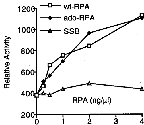
Figure 6. RPA purified from mock-treated cells (wt-RPA) and from adozelesin-treated cells (ado-RPA) were tested in polymerase assays. The DNA template is a long single-stranded DNA with only adenosine (poly dA) annealed with a short oligonucleotide with only thymidine (oligo dT). DNA polymerase \alpha and radioactive labeled dTTP were used to label newly synthesized DNA. While RPA is not essential for this reaction, the presence of RPA greatly stimulate the polymerase activity, which can not be replaced by SSB.
