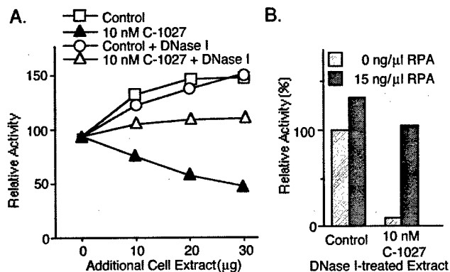
FIGURE 5: DNase I treatment eliminates the trans inhibitor in extracts from cells treated with high levels of C-1027. (A) 40 \mu\text{g} of extract from mock-treated cells was mixed with 0–30 \mu\text{g} of DNase I-treated extract from mock- or 10 nM C-1027-treated cells. These mixtures were then tested for the ability to support in vitro DNA replication. In three independent experiments, the addition of 30 \mu\text{g} of extract from cells treated with 10 nM C-1027 resulted in >40% inhibition of DNA replication by 40 \mu\text{g} of control cell extract. The addition of 30 \mu\text{g} of the same extract first treated with DNase I to 40 \mu\text{g} of control cell extract always showed DNA synthesis levels greater than that seen with 40 \mu\text{g} of control cell extract alone. (B) 0 or 15 ng/ \mu\text{L} purified RPA was added to SV40 DNA replication assays carried out with 40 \mu\text{g} of DNase I-treated extracts from either mock- or 10 nM C-1027-treated cells. In three independent experiments, the level of DNA replication by 40 \mu\text{g} of extract from cells treated with 10 nM C-1027 was always < 10% of levels seen with 40 \mu\text{g} of control cell extract. Addition of 15 ng/ \mu\text{L} RPA to 40 \mu\text{g} of extract from cells treated with 10 nM C-1027 resulted in DNA replication levels of 90–110% of that seen with 40 \mu\text{g} of control cell extract. Relative activity (%) indicates the percent of DNA synthesis seen in comparison to levels of synthesis seen with the control reaction, 40 \mu\text{g} of untreated extract from mock-treated cells with no additional RPA.
