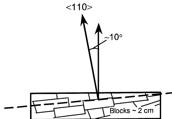
Figure 3. Structure and orientation of silicon block from which the samples were cut off.
