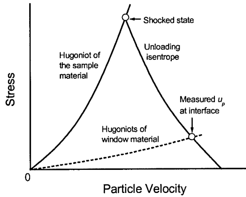
Figure 7. Decomposition of shock discontinuity at interface between the sample and the window.
