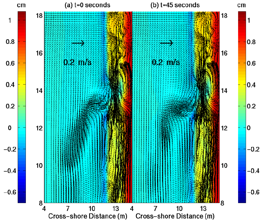
Fig. 16 — Laboratory domain: Snapshots of the ADCIRC water levels and currents for the unsteady rip current at (a) t = 0 s and (b) t = 45 s. Arrows representing a 0.2 m/s current indicate the magnitudes of the current field vectors. Note: Only every third current vector of the current vector field is plotted.
