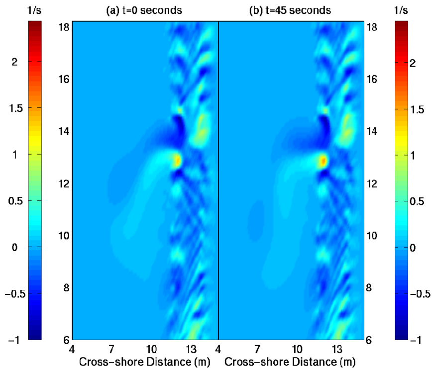
Fig. 17 — Laboratory domain: Snapshots of the unsteady rip current vorticity (determined from the ADCIRC solution for the velocity) at (a) t = 0 s and (b) t = 45 s.
