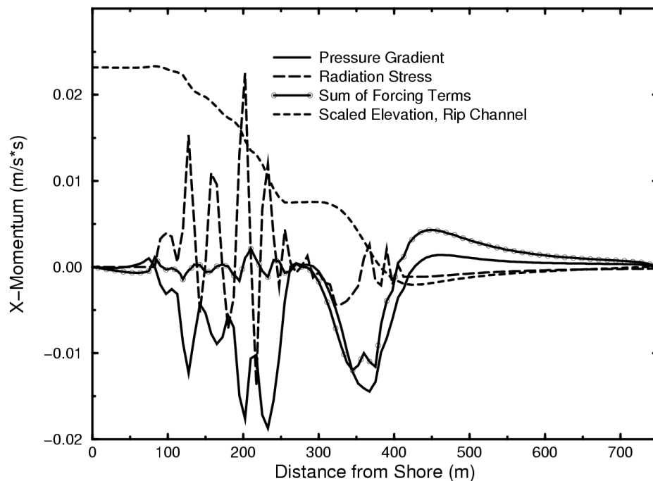
Fig. 7 — Ideal barred beach: Cross-shore transects along the rip channel ( y = 750 m) of the steady-state, cross-shore-directed pressure gradient, radiation-stress gradient, and sum of all the cross-shore-directed forcing terms. The scaled steady-state elevation is also depicted in order to see the correspondence between it and the forcing terms.
