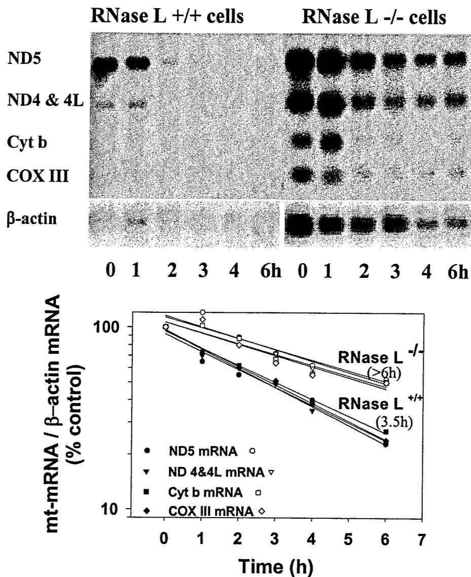
Figure 4. Mitochondrial transcripts are stabilized in RNase L ^{-/-} cells. Total cytosolic RNA was isolated from RNase L ^{+/+} and RNase L ^{-/-} mouse embryo fibroblasts at indicated time points after termination of transcription by actinomycin D, and 2 \mu g aliquots were subjected to Northern blot analysis as described under "Materials and Methods". Hybridization was quantified by image analysis of autoradiograms. Semi-log plots of transcript remaining versus time is depicted in case of \beta -actin mRNA.
