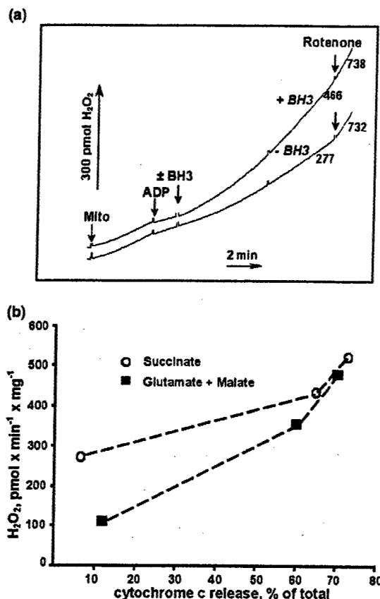
Fig. 6 Stimulation of cytochrome c release and H_2O_2 production by brain mitochondria by addition of Bax plus a BH3 domain peptide. Mitochondria were added at a concentration of 0.125 mg/mL to the standard incubation medium maintained at 37°C and supplemented with either 5 mM glutamate and 5 mM malate or 5 mM succinate. (a) Amplex Red measurements of H_2O_2 generation. At approximately 3 min following addition of brain mitochondria to media containing glutamate and malate and 100 nM Bax (see Materials and methods), 0.1 mM ADP was added to initiate State 3 respiration. Approximately 2 min later, 50 \mu M BH3 peptide or vehicle control ( H_2O ) was added. Rotenone (0.2 \mu M) was added 9 min later to elicit maximal H_2O_2 production. (b) Relationship between H_2O_2 production and release of cytochrome c caused by exposure of brain mitochondria to Bax plus a BH3 peptide. In experiments such as that shown in (a) aliquots of the mitochondrial suspension were removed before and two or three times after addition of the BH3 peptide or vehicle, centrifuged and used for ELISA of cytochrome c release from the mitochondria into the medium. The corresponding rate of H_2O_2 production refers to the rate obtained just before removal of the aliquot for cytochrome c measurement. Experiments were performed either in the presence of 5 mM succinate (○) or 5 mM glutamate and 5 mM malate (■).
