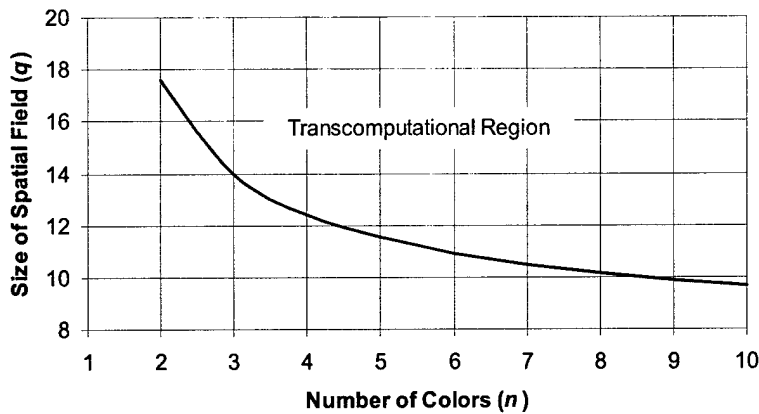
Figure 6. The Bremermann's Limit for Pattern Recognition
