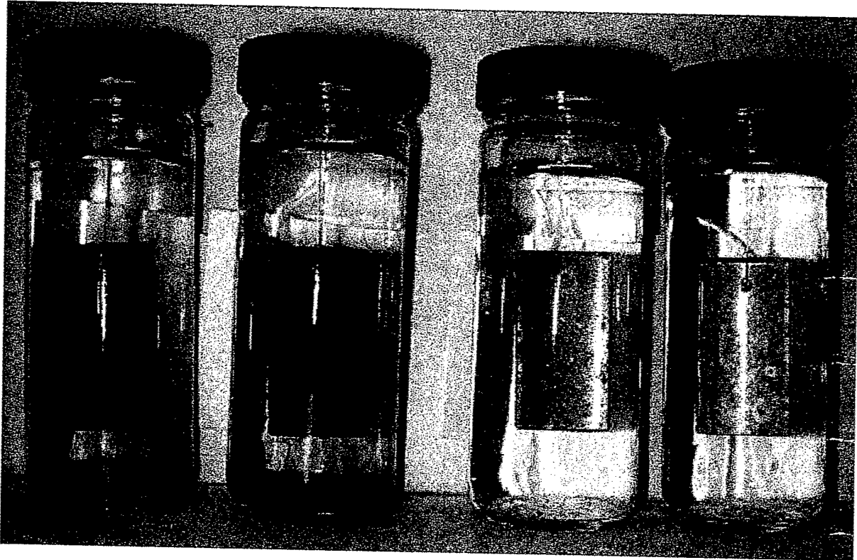
Figure 1. Test set-up for evaluating the influence of inhibitor additives on corrosion processes in seawater. Sample bottles from left to right, 1018 steel in 1/4 and 1/2 strength seawater, 6061 aluminum in 1/4 and 1/2 strength seawater.
