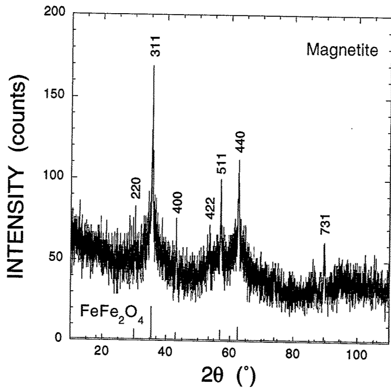
Figure 10. X-ray diffraction spectrum of corrosion product formed on the surface of steel coupon immersed in seawater containing ADD6 inhibitor. Superimposed are the reflections of the FeFe 2 O 4 standard.
