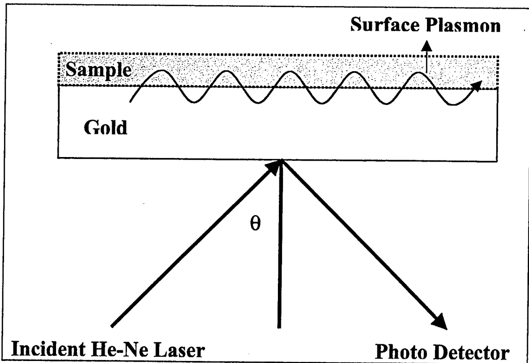
Figure 3. Schematic diagram describing SPR measurement and interpretation of results.
