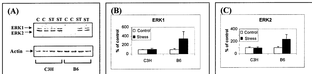
Figure 2. Effect of shear stress on phosphorylation levels of MAPK in osteoblasts isolated from C3H and B6 mice. Cells were subjected to fluid flow of 20 dynes/cm 2 for 30 minutes. (A): Cell lysates were immunoblotted with anti-phospho-ERK and anti-actin antibodies. (B&C): The graph represents the densitometric measurements of ERK1 and ERK2 phosphorylation levels from western blots normalized by actin.
