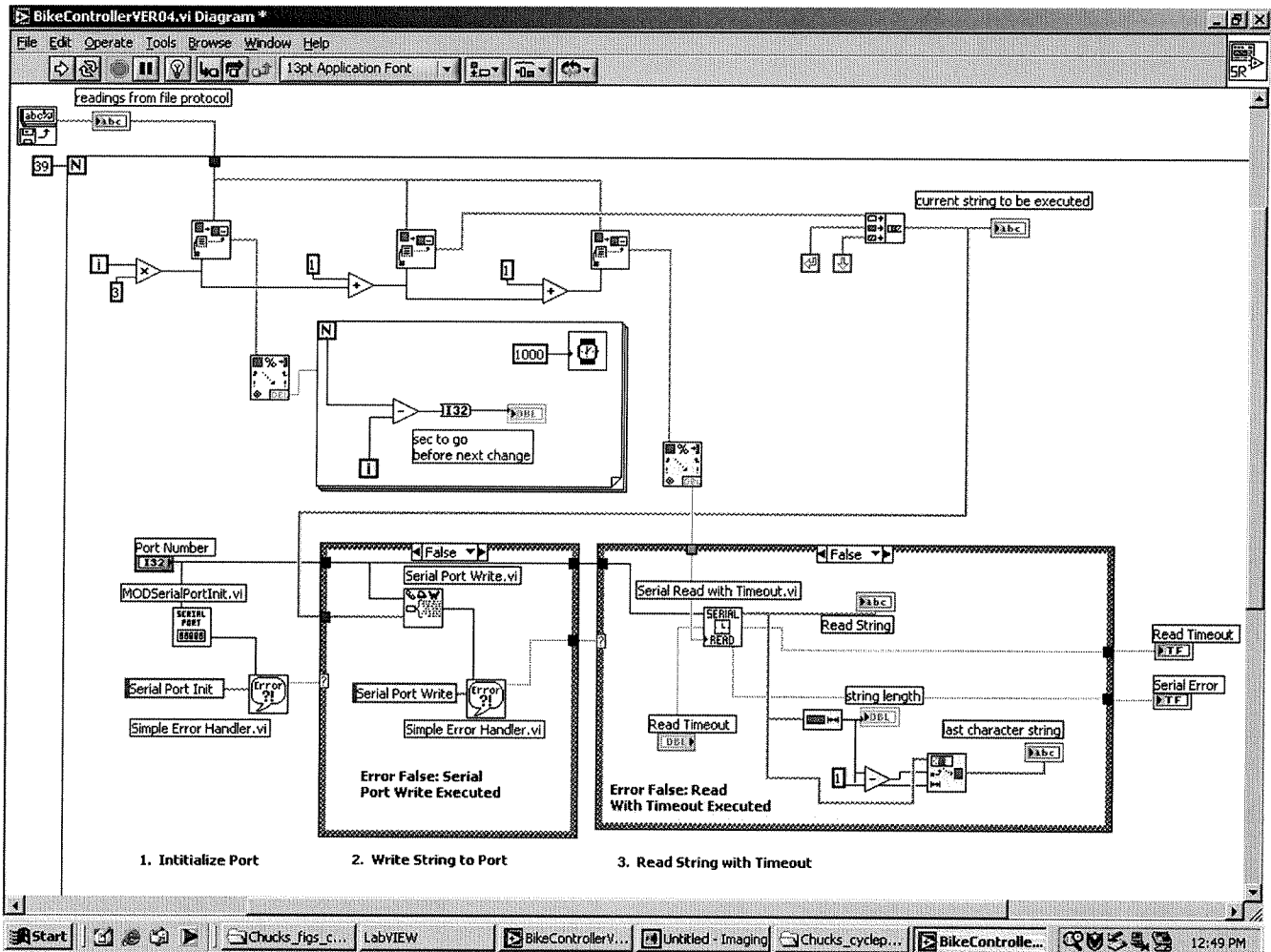
FIGURE 9: Diagram of BikeController. This part of the diagram is devoted to handle operations related to sending commands to the Cardio2 Cycle and then reading the responses via the serial port.
