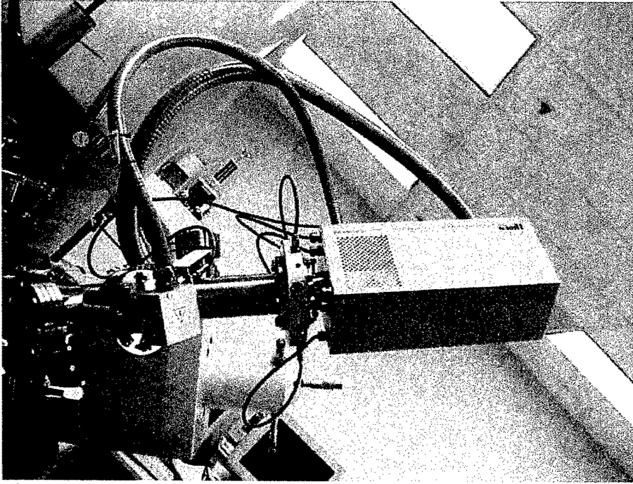
Figure 2: Hiden Quadrupole SIMS Analyzer
