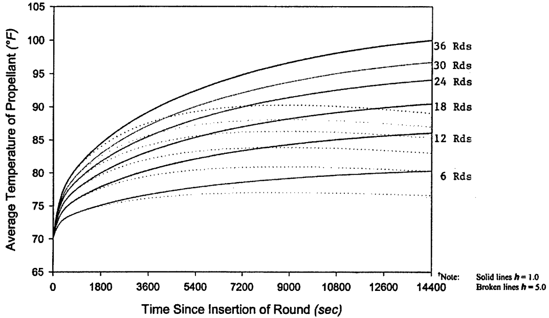
Figure 6. Propellant average temperature versus time with mild crew compartment temperature and mild round temperature at h equals 1.0 and 5.0.
