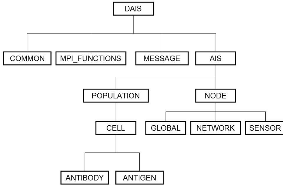
Figure 32 DAIS Object Relational Diagram
