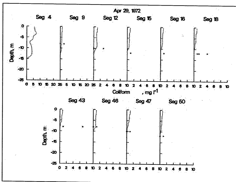
Figure 6-68. Average conditions calibration profile coliform
