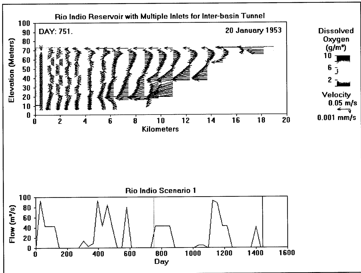
Figure 7-76. Rio Indio Reservoir main branch dissolved oxygen day 751 of simulation, inter-basin transfer with multiple tunnel inlets
