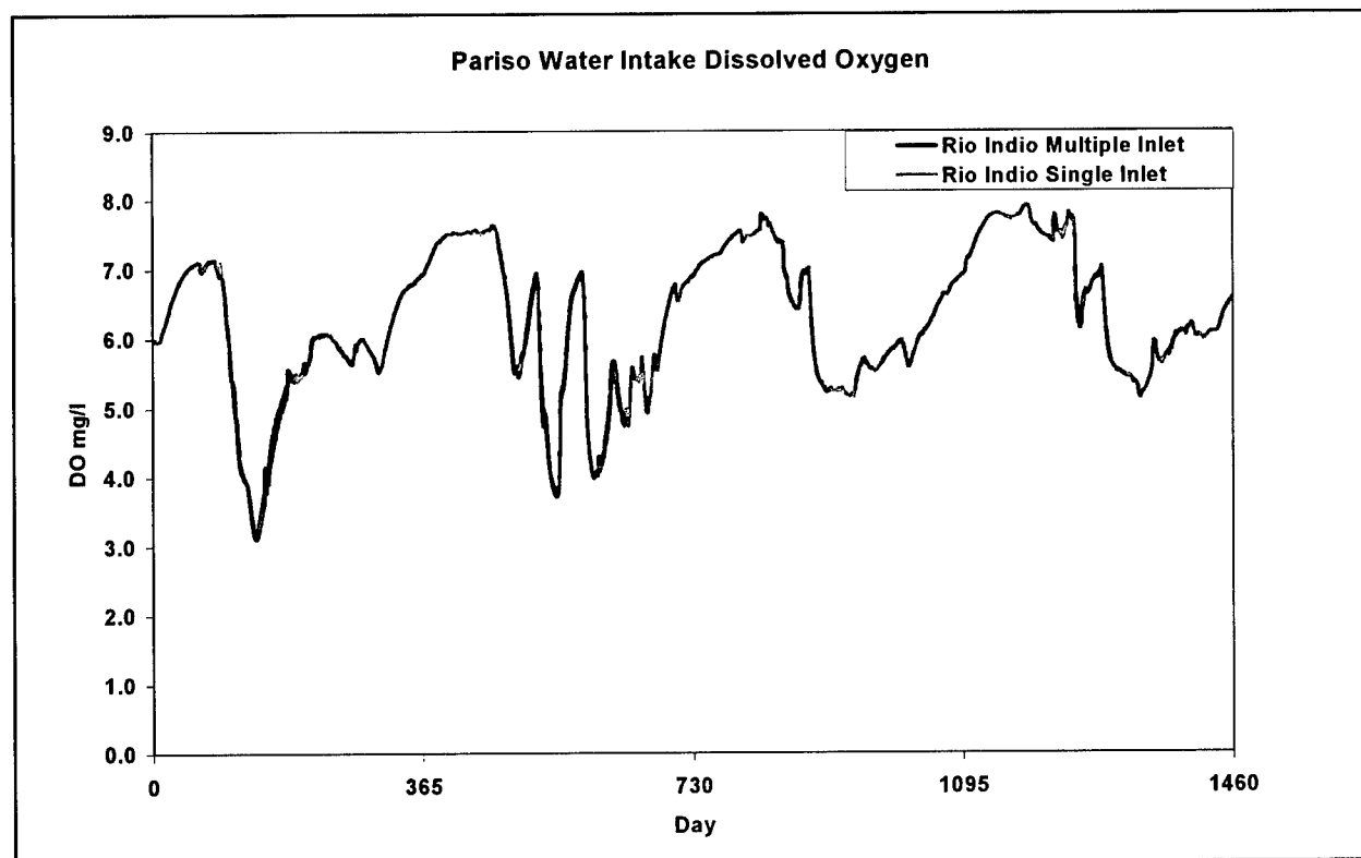
Figure 7-84. Parisio water intake dissolved oxygen
