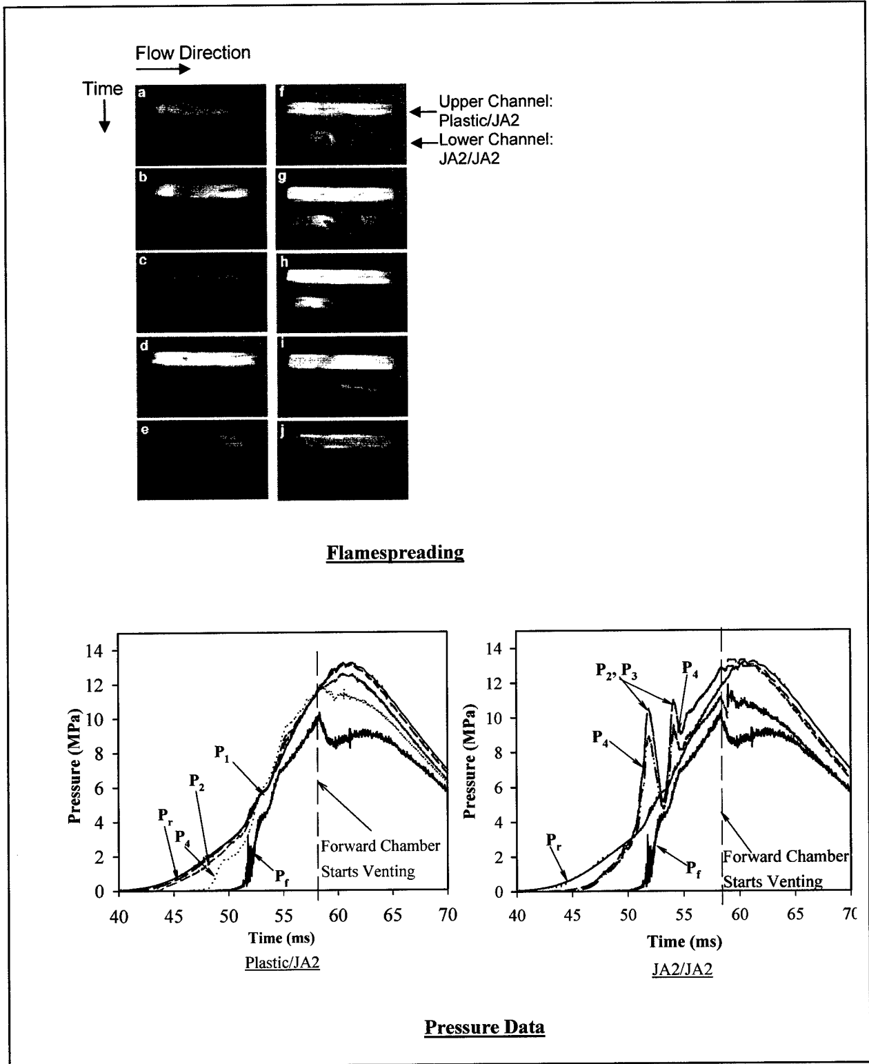
Figure 6. Run 4: W = 0 mm for both channels (open end); plastic/JA2 vs. JA2/JA2.
