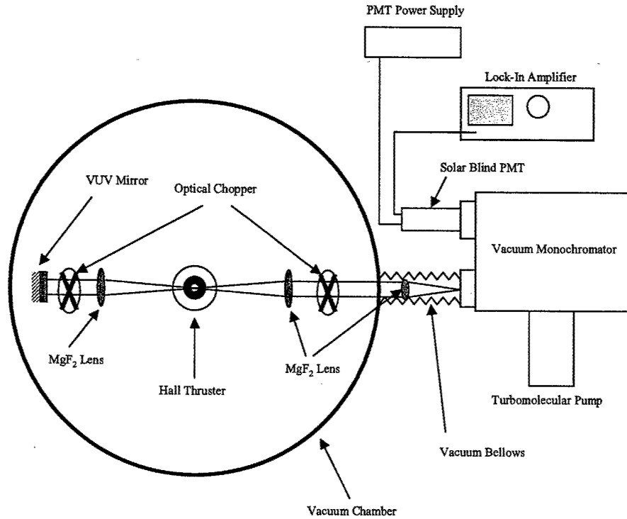
Figure 4: Experimental Schematic.
