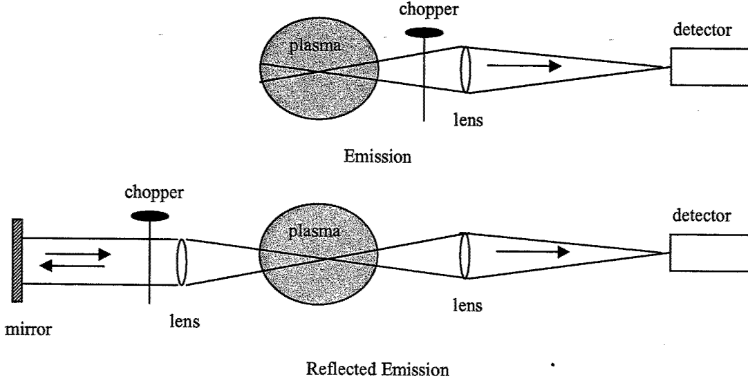
Figure 1: (a) top-conventional emission measurement. (b) bottom-absorption of the reflected emission, redirected through the plasma opposite the direction of the direct emission.
