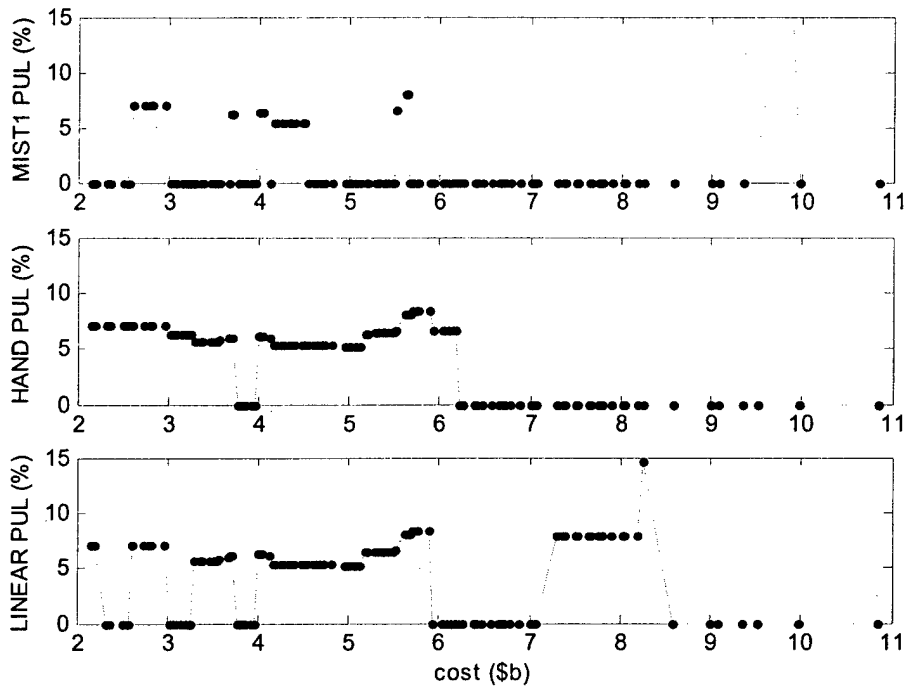
Figure 29: Proportional Utility Loss (PUL) for Alternate Utility Sets -- No Weighting
