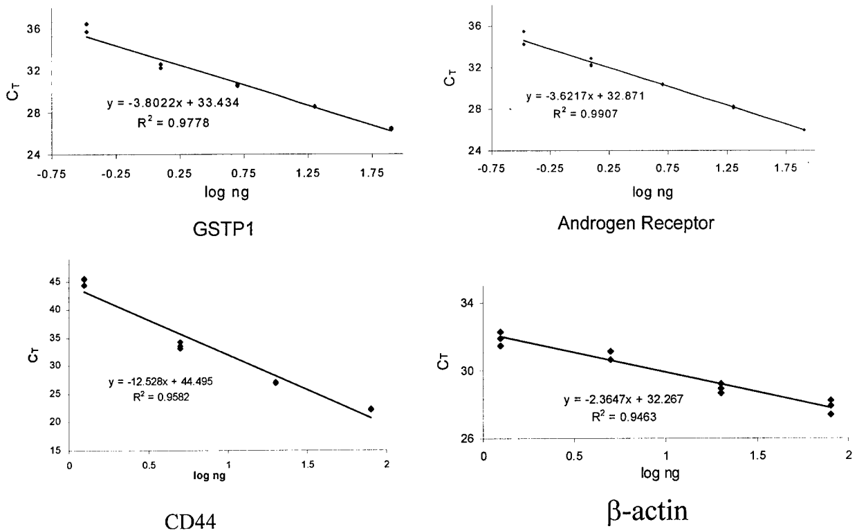
Figure 1. Real time PCR for candidate genes - standard plot. Varying quantities of human placental DNA (80ng, 20ng, 5ng, 1.25ng) was used as template in triplicate for the real time PCR. The threshold values ( C_T ) were plotted against the log ng of input DNA and the regression equation so generated can be used to quantitate the input quantity of DNA from an unknown sample by using the threshold value.
