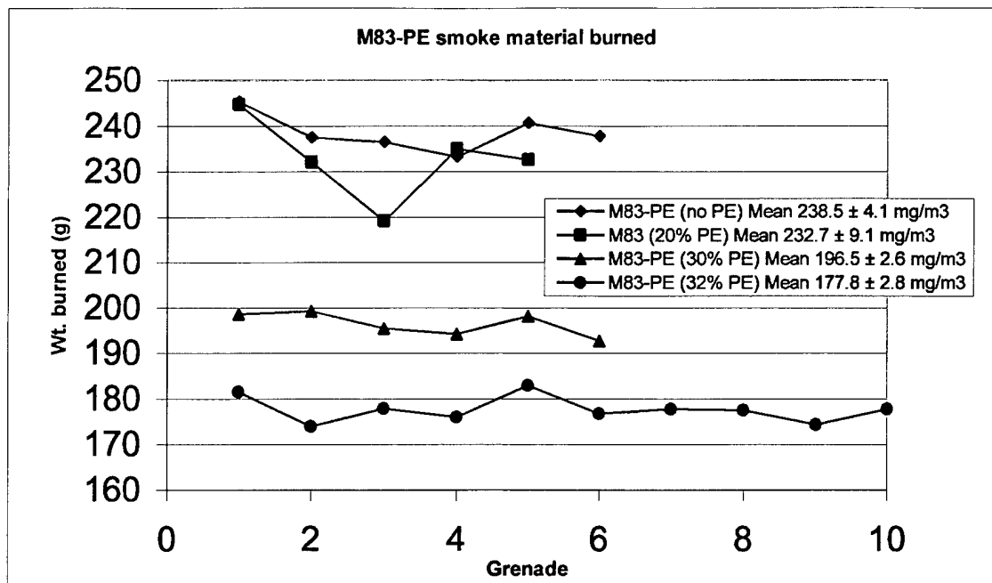
Figure 3. Weight (g) of smoke material burned from M83-PE grenades.
