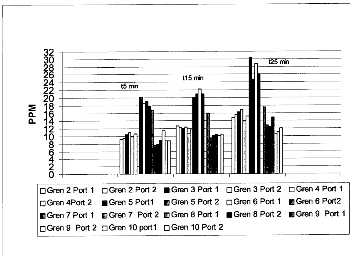
Figure 6. Benzene concentrations from 300-liter chamber.
