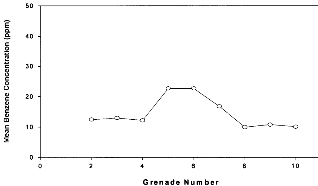
Figure 8. Mean benzene concentrations (ppm) vs. grenade number.
