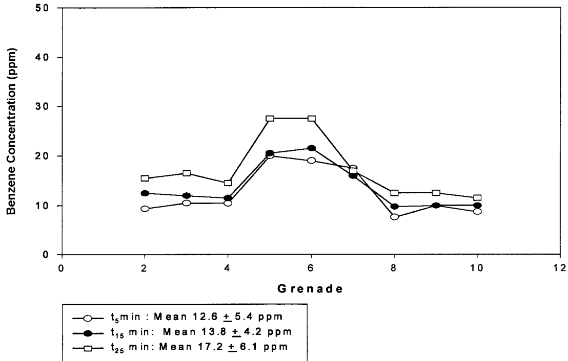
Figure 7. Benzene concentrations vs. grenade at t_5 , t_{15} , and t_{25} minutes.
