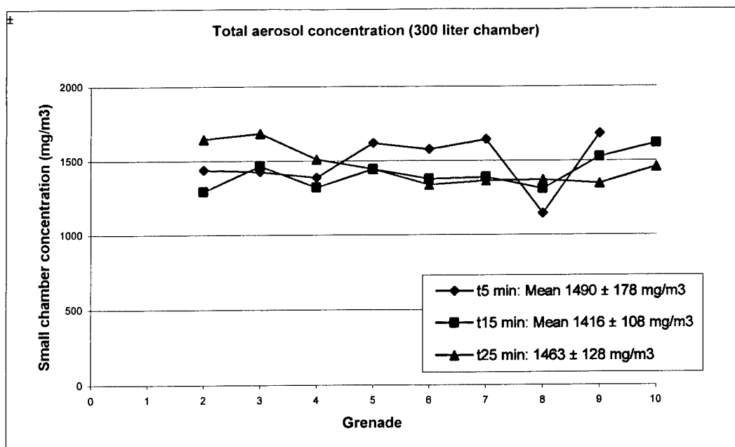
Figure 5. 300-liter chamber concentrations (mg/m 3 ) taken at t 5 , t 15 , and t 25 minutes.
