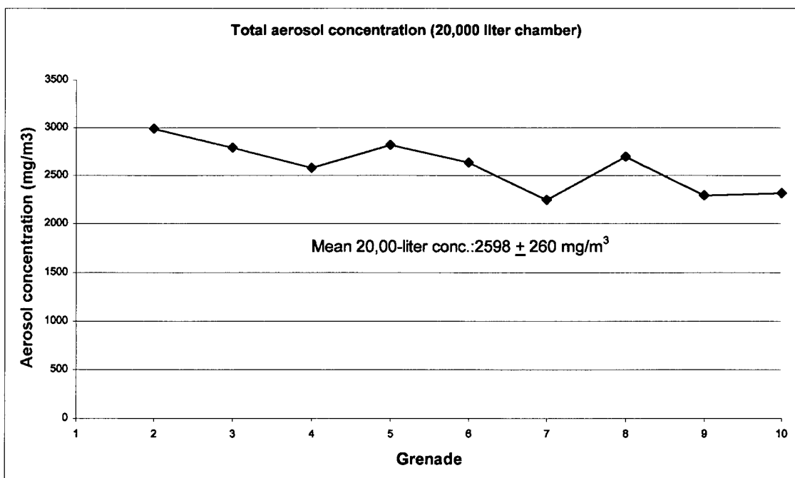
Figure 4. 20,000-liter chamber concentrations (mg/m 3 ) taken at t_7 minutes.
