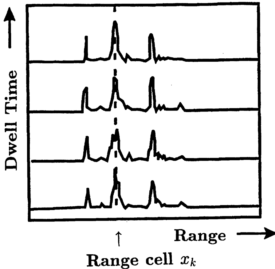
Figure 1: Range profiles versus dwell time (or pulse number) after coarse range alignment.
