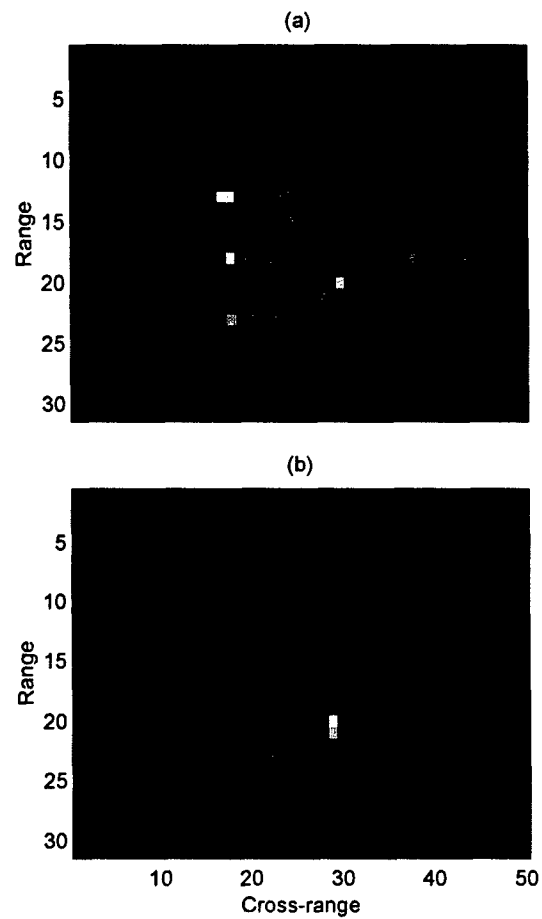
Figure 7: ISAR image formation from experimental radar data: (a) ISAR image of measured corner reflectors using conventional Fourier transform; (b) resulting final image after residual rotational motion compensation.
