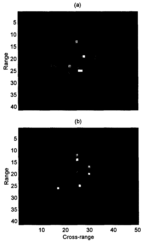
Figure 10: ISAR image formation from experimental radar data: (a) ISAR image of measured corner reflectors using conventional Fourier transform; (b) resulting final image after residual rotational motion compensation.
