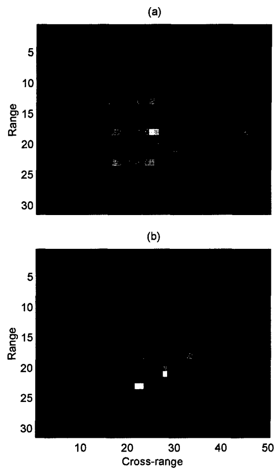
Figure 6: ISAR image formation from simulated corner reflectors data: (a) ISAR image of simulated corner reflectors using conventional Fourier transform; (b) resulting final image after rotational motion compensation.
