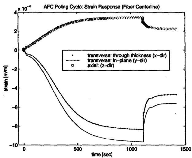
Figure 5-8: Fiber centerline strains.
