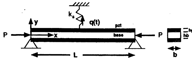
Figure 2-5: Model of bender structure being analyzed.
