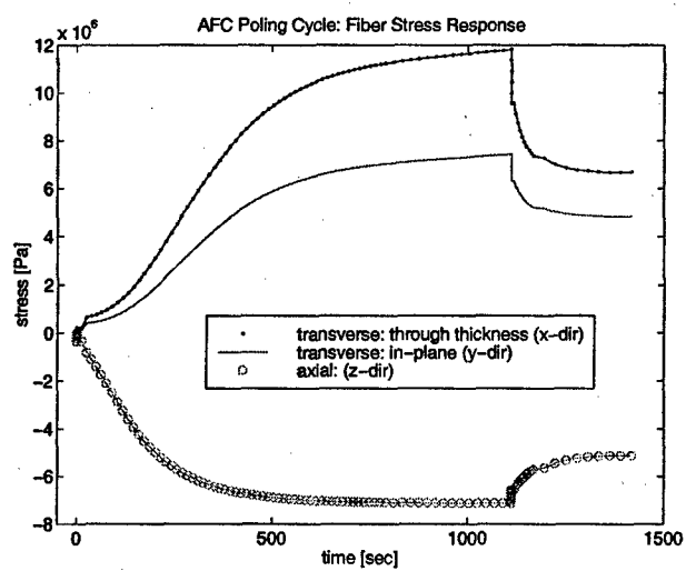
Figure 5-10: Fiber centerline stress response.
