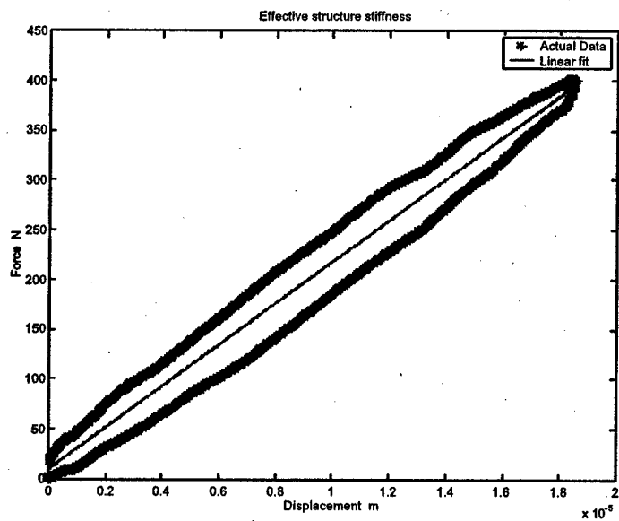
Figure 4-23: Typical Effective Stiffness Determined from Actual Data
