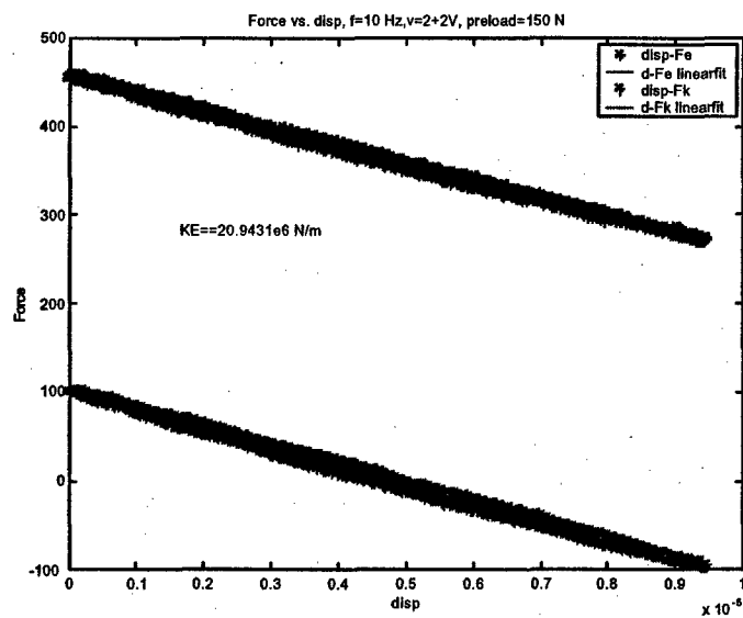
Figure 4-6: Force vs. Displacement for Stack Stiffness Measurement
