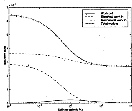
Figure 2-9: Work in and work out expressions plotted for varying values of stiffness ratio. Values plotted are the maximum work values over a cycle with 100 V maximum input voltage.
