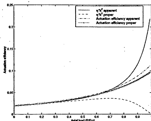
Figure 2-6: Actuation efficiency and device coupling coefficient against the mechanical preload of the system, plotted for \frac{k_2}{K} = 0.7 .
