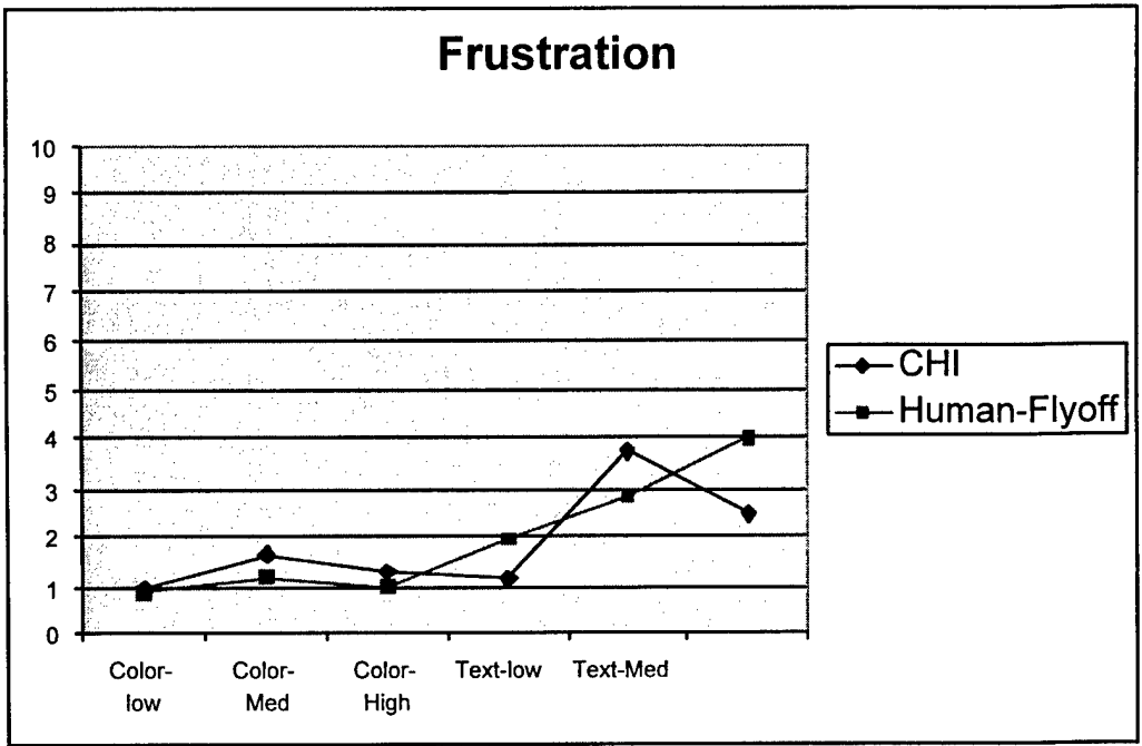
Figure 3-14. Model versus Human Subjects on Frustration Measures
