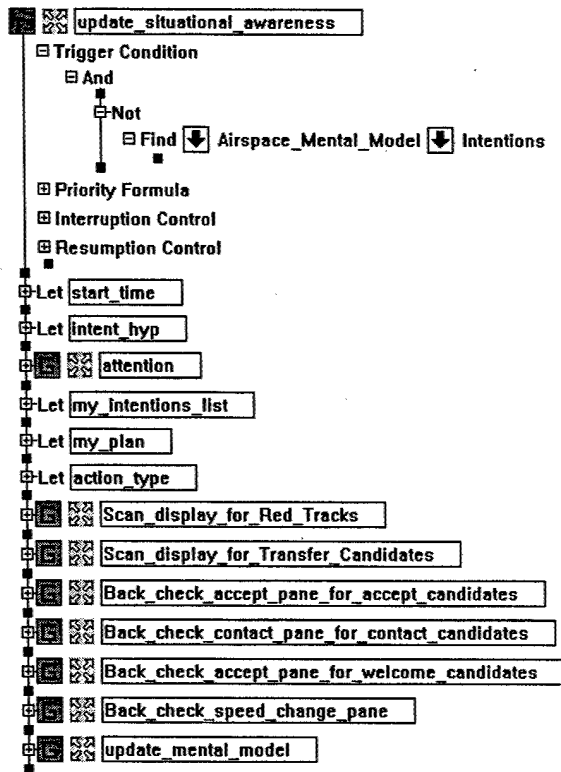
Figure 3-5. High-level View of SA Task
