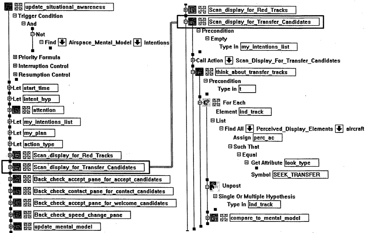
Figure 3-6. Update Situation Awareness Task Extract
