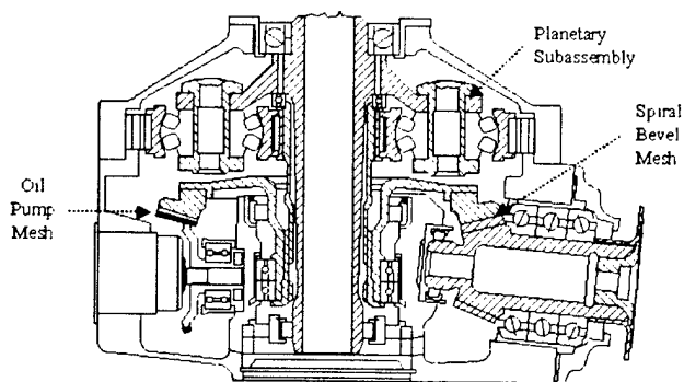
Figure 1. OH-58 Main Rotor Transmission
