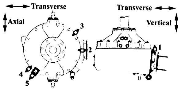
Figure 4. Accelerometer locations
