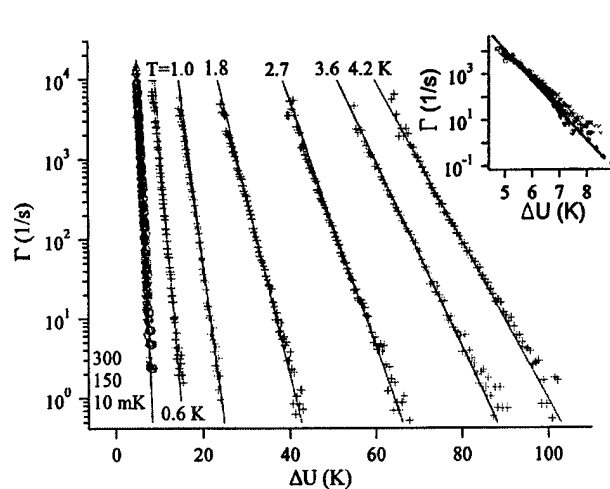
FIG. 3. Tunneling rates vs potential barrier at various temperatures. The symbols are data and the solid lines are theoretical predictions. The first three data sets from the left are T = 10 \text{ mK} (triangles), 150 \text{ mK} (circles), and 300 \text{ mK} (crosses). Inset: The measured (symbols) and predicted (lines) tunneling rates vs barrier height for T = 10 \text{ mK} (triangles and solid line), 150 \text{ mK} (circles and dotted line), and 300 \text{ mK} (crosses and dashed line).
