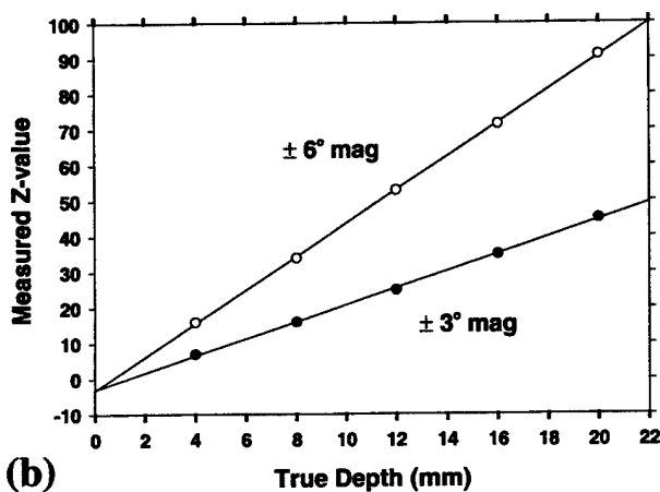
FIG. 3. (a) Calibration lines for ±3° stereo shift contact and ±6° stereo shift contact acquisition; (b) calibration lines for ±3° stereo shift magnification and ±6° stereo shift magnification acquisition.
