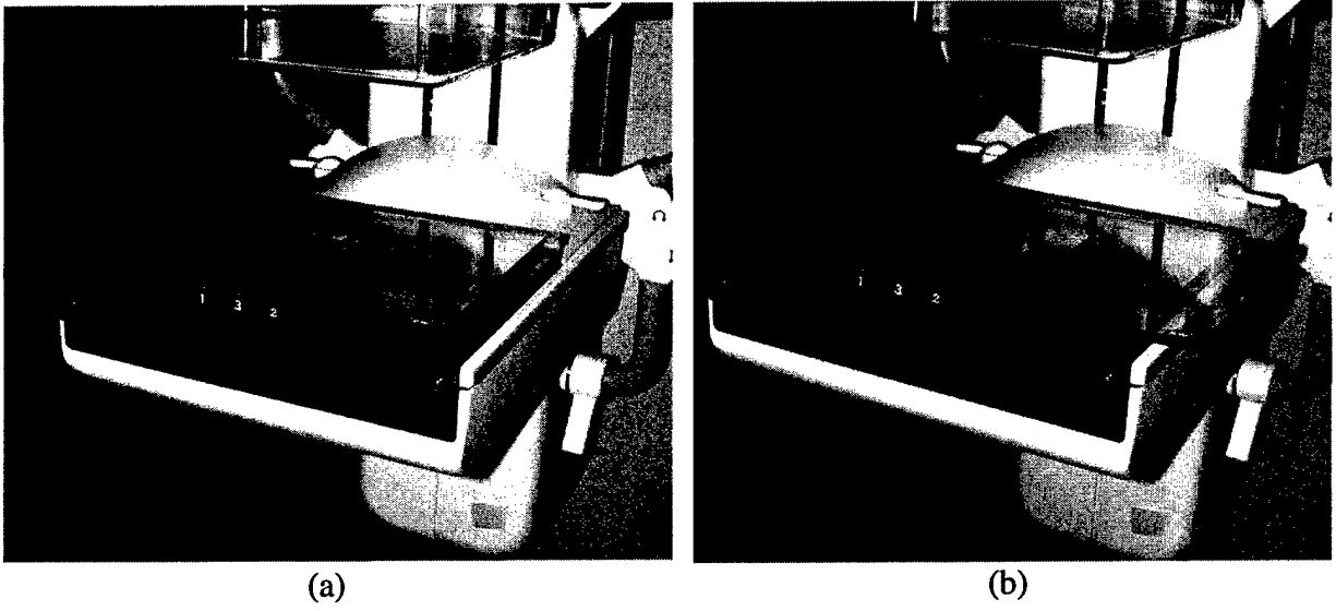
Fig. 3. The phantom platform placed on top of the detector of the digital mammography system in the setup for contact imaging. The sliding plate with the stereo phantom was shifted to the left in (a) and to the right in (b) at a distance equivalent to a \pm 3^\circ stereo angle.
