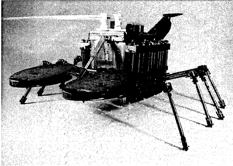
Figure 3.1: Lobster Robot
