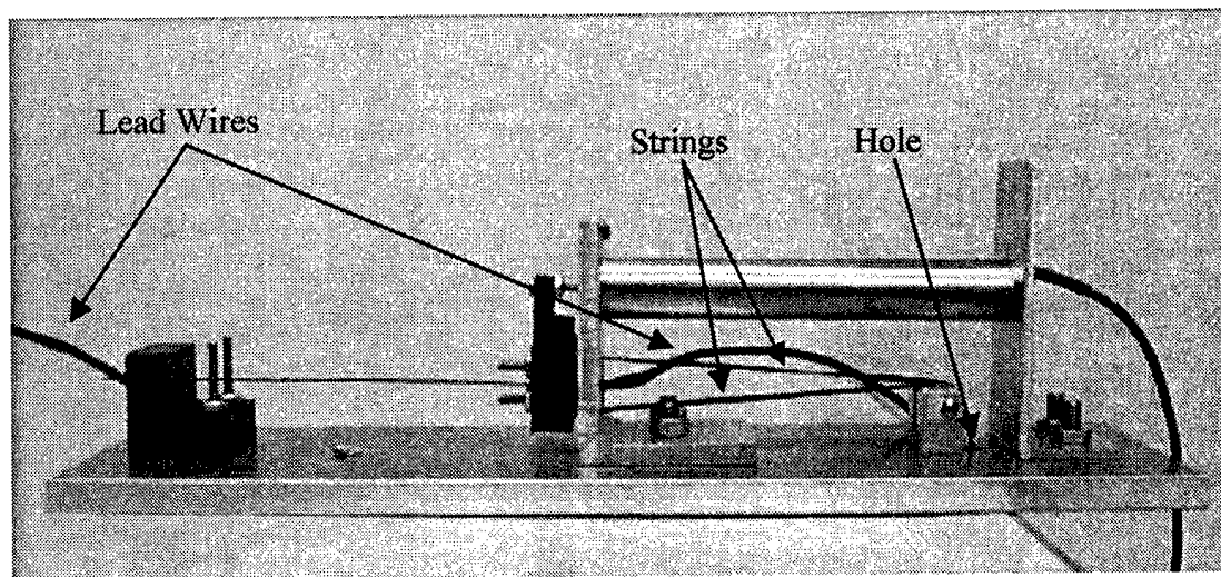
Figure 6.5: Test Fixture
