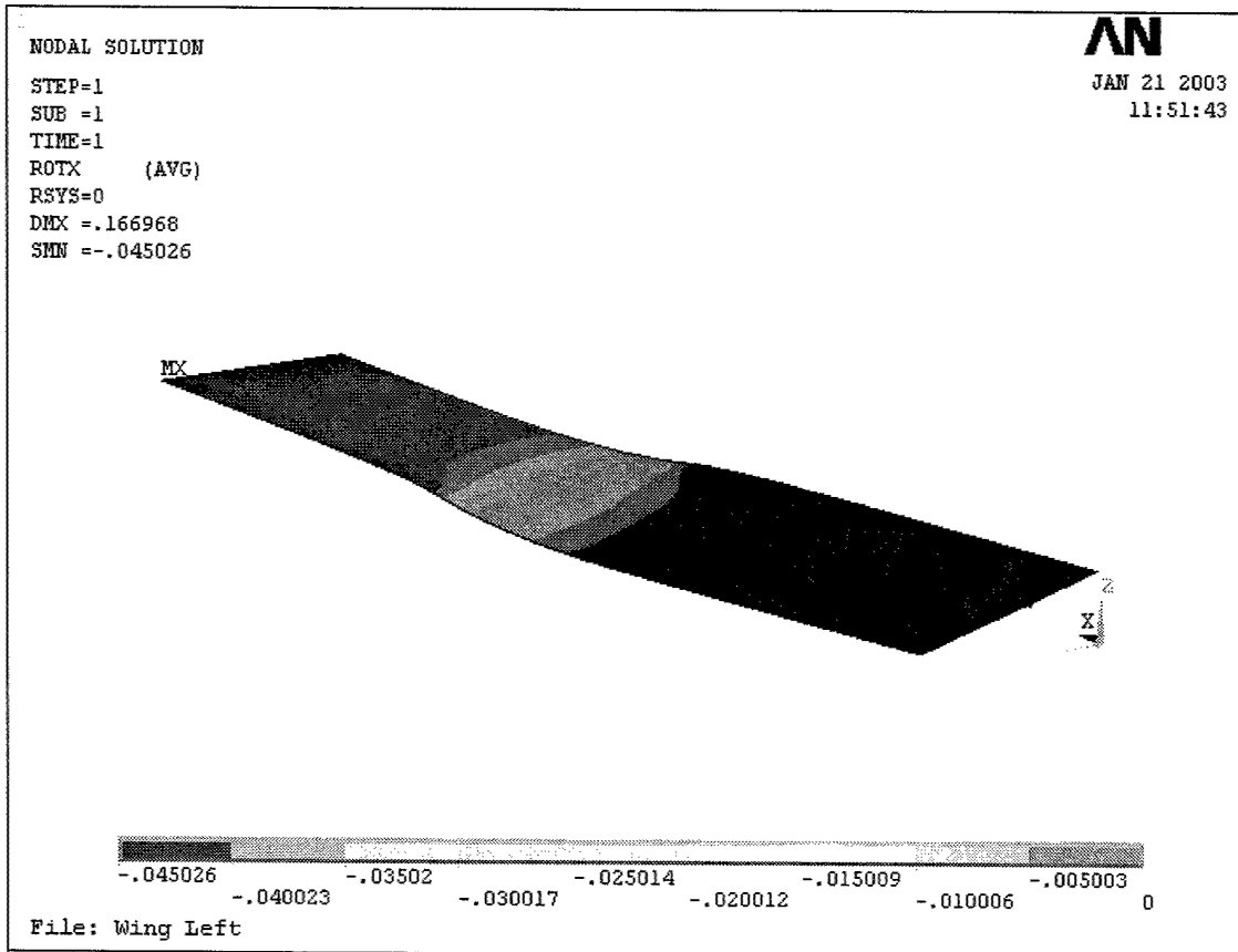
Figure 5.12: Rotation Results for Configuration 3
