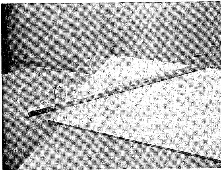
Figure 7.5: Pre-straining Fixture
