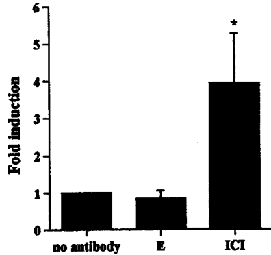
Figure 6 ChIP assay demonstrates increased transcription following stimulation by ICI. MCF-7 cells were treated for 48 h with 10 -7 M 17β-estradiol in the absence of serum. Cells were washed twice with IMEM and stimulated for 2 h with 10 -8 M ICI. An antibody to RNA PoIII was used for immunoprecipitation and a fragment of AIB1 exon 4 was amplified and quantified by real time PCR. The amount of AIB1 DNA pulled down by IP was corrected for the amount of DNA in the input. The no antibody control indicates background levels of AIB1 pulled down non-specifically during IP and was arbitrarily set at 1. The amount of AIB1 DNA pulled down in the estradiol and ICI treated cells is expressed as fold induction over the background no antibody control. Results are based on at least three separate experiments; error bars represent s.e.m. Statistical analyses were performed using a t -test. * P < 0.05 compared to untreated cells
