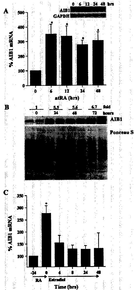
Figure 4 All-trans retinoic acid increases AIB1 gene expression and is reversed with estradiol. (a) MCF-7 cells were grown in full media for 24 h and then treated with 10^{-6} M atRA in serum-free media and the cytoplasmic RNA was harvested over 48 h. Following Northern blot analysis, AIB1 levels were analysed by phosphorimager and corrected by GAPDH. Untreated cells (0 h) were arbitrarily set at 100% and treated cells were analysed in reference to this. Results are based on five separate experiments; error represent s.e.m. Statistical analyses were performed using a t -test. *P < 0.05 compared to untreated cells. Inset represents a typical Northern blot. (b) MCF-7 cells were grown in full media for 24 h and then treated with 10^{-6} M atRA in serum-free media for 24, 48, and 72 h. Cell lysates were harvested and subjected to Western blot analysis using an anti-AIB1 antibody. Ponceau S staining was used as a loading control. Relative fold changes in AIB1 are indicated numerically above lanes. (c) MCF-7 cells were grown in full media and treated with 10^{-6} M atRA in serum-free media for 24 h, washed twice with IMEM followed by treatment with 10^{-7} M 17\beta -estradiol in serum-free media and the cytoplasmic RNA was harvested over 48 h. Following Northern blot analysis, AIB1 levels were analysed by phosphorimager and corrected by GAPDH. Untreated cells (–24 h) were arbitrarily set at 100% and treated cells were analysed in reference to this. Results are based on at least three separate experiments; error bars represent s.e.m. Statistical analyses were performed using a t -test. *P < 0.05 compared to untreated cells. Vehicle control (DMSO and EtOH) showed no statistical difference from untreated cells (data not shown)
