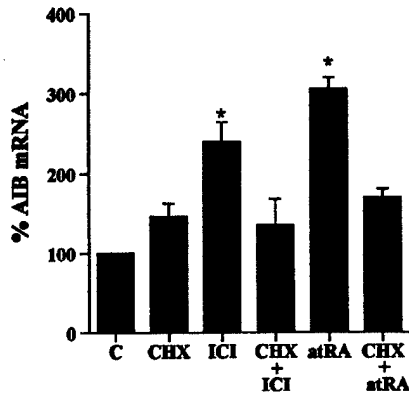
Figure 7 De novo protein synthesis is necessary for the induction of AIB1 mRNA by ICI and atRA. MCF-7 cells were treated with 10 μg/ml cycloheximide (CHX) alone and in the presence of 10 -8 M ICI or 10 -6 M atRA and the cytoplasmic RNA was harvested after 24 h. Following Northern blot analysis, AIB1 levels were analysed by phosphorimager and corrected by GAPDH. Untreated control cells (C) were arbitrarily set at 100% and treated cells were analysed in reference to this. Results are based on at least three separate experiments; error bars represent s.e.m. Statistical analyses were performed using a t -test. * P < 0.05 compared to untreated cells
