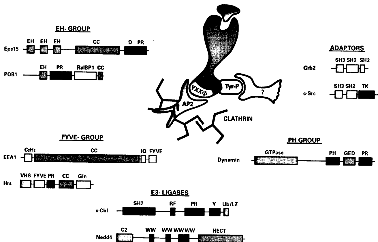
Fig. 2. Molecules involved in sorting RTKs along the endocytic pathway. The transmembrane receptor is schematically depicted in a complex with AP2 and a clathrin cage. The interaction of AP2 with the cytoplasmic part of the receptor is mediated by an endocytic signal such as the YXXΦ motif, but other adapters, whose engagement depends on tyrosine phosphorylation, may enhance recruitment of the AP2 complex. Molecules involved in this sorting event, as well as the sorting that occurs in multi vesicular bodies are grouped and schematically presented. The structural domains are shown in different colors and their names indicated. The abbreviations used are: CC, coiled coil; C2, a phospholipid and calcium binding region; D, a region containing DPF repeats; EH, Eps15 homology; FYVE, a PI3P binding; RF, a RING finger domain; PR, a proline-rich domain; SH, Src homology domain; TK, tyrosine kinase.
