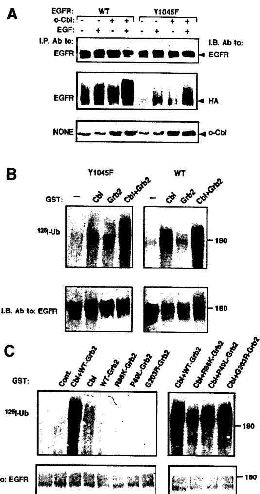
Fig. 4. An alternative receptor ubiquitylation pathway independent of Tyr1045 may involve Grb2. (A) CHO cells were transfected with plasmids encoding a wt-EGFR (WT) or the Y1045F mutant, along with vectors encoding c-Cbl and an HA-tagged ubiquitin. Following 48 h, cell monolayers were treated for 10 min at 37°C without or with EGF (100 ng/ml) and cell lysates subjected to immunoprecipitation (I.P.) and immunoblotting (I.B.) with the indicated antibodies. Whole-cell lysates were also analyzed (lower panel). (B) wt-EGFR or the Y1045F mutant receptor were immunoprecipitated from transfected HEK-293 cells. Receptor immunoprecipitates were subjected to an in vitro ubiquitylation assay with a radiolabeled ubiquitin. c-Cbl, Grb2 or a combination of the two proteins was added to the reaction mixtures in the form of GST fusion proteins. Receptor immunoprecipitates were resolved by electrophoresis and proteins transferred to filters, which were first autoradiographed (upper panel, ^{125} I-Ub) and then immunoblotted with anti-EGFR antibodies (lower panel). (C) Immunoprecipitates of Y1045F were subjected to an in vitro ubiquitylation assay in the presence of one or two of the indicated GST fusion proteins. As a control, GST was added alone (Cont.) or it was omitted from the reaction (unlabeled lane).
