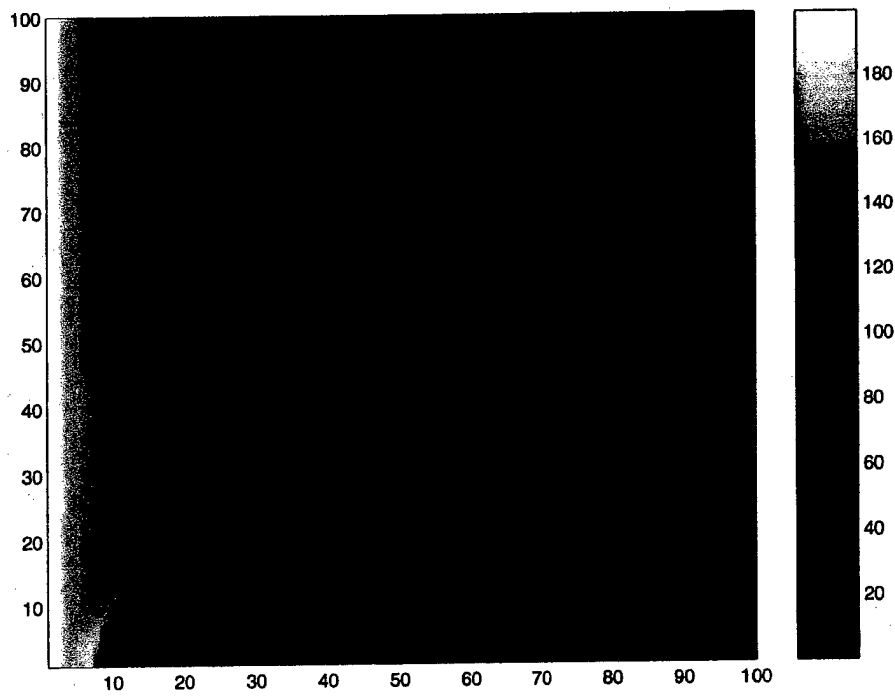
Figure 5.27: Variance of surface
