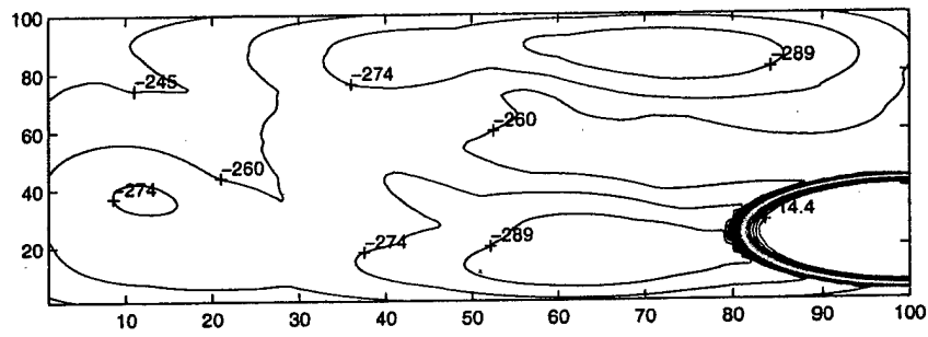
Figure 5.24: Negative variance of bottom topography
