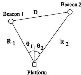
Figure 4. The platform and the two beacons projected on a horizontal plane.
