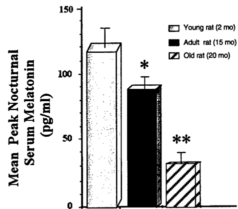
Figure 2. Peak daytime and nighttime serum levels of melatonin in adult and young female Buffalo rats. Serum melatonin levels of 10 young (2 months of age), 10 adult (15 months of age) and 10 old (20 months of age) female Buffalo rats at 2400 h (dark phase). Animals were maintained in a light:dark cycle of 12:12 before being killed under a red-light. * p < 0.05 vs. young rats.
