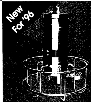
Integrated MK3C CTD and Compact Rosette System Capacities ranging from 500 ml to liter bottles
