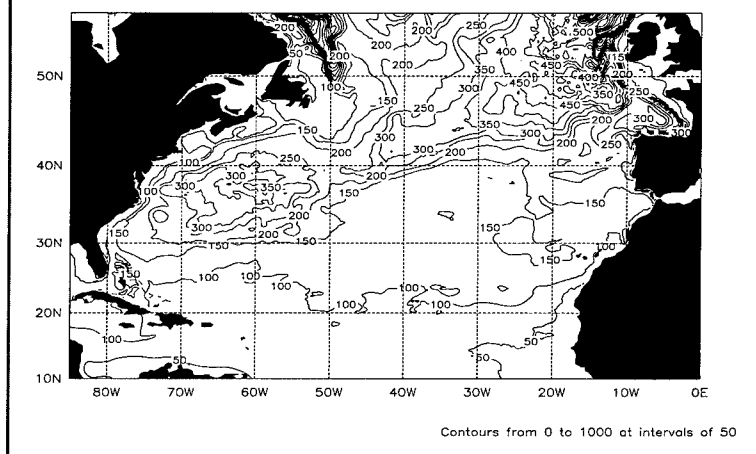
A simulation of mixed layer depth (in meters) in the North Atlantic using an isopycnic coordinate model 5 . Mixed layer depth predictions are required for forecasting acoustic surface duct conditions and assessing the performance of RN sonars.
