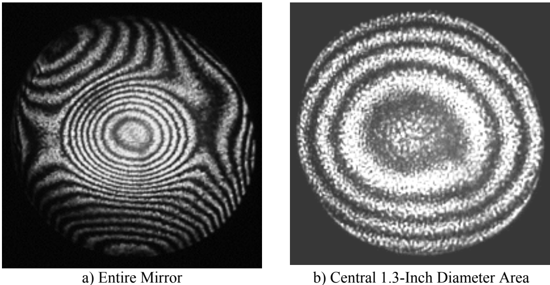
Figure 7-5. ZYGO Interferometer Images of Initially Flat CP1 Polymer Substrate Suspended on an Aluminum Mounting Ring [2]
