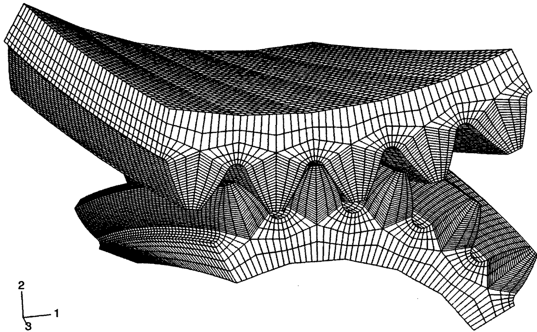
Figure 3.—Contacting model of five pairs of teeth derived for stress analysis.
