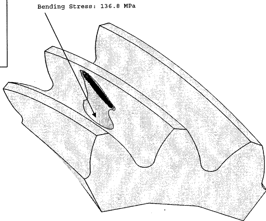
Figure 32.—Contact and bending stresses in the middle point of the path of contact on pinion tooth surface for modified involute helical gear drive wherein the generation is performed by plunging of the grinding worm.
