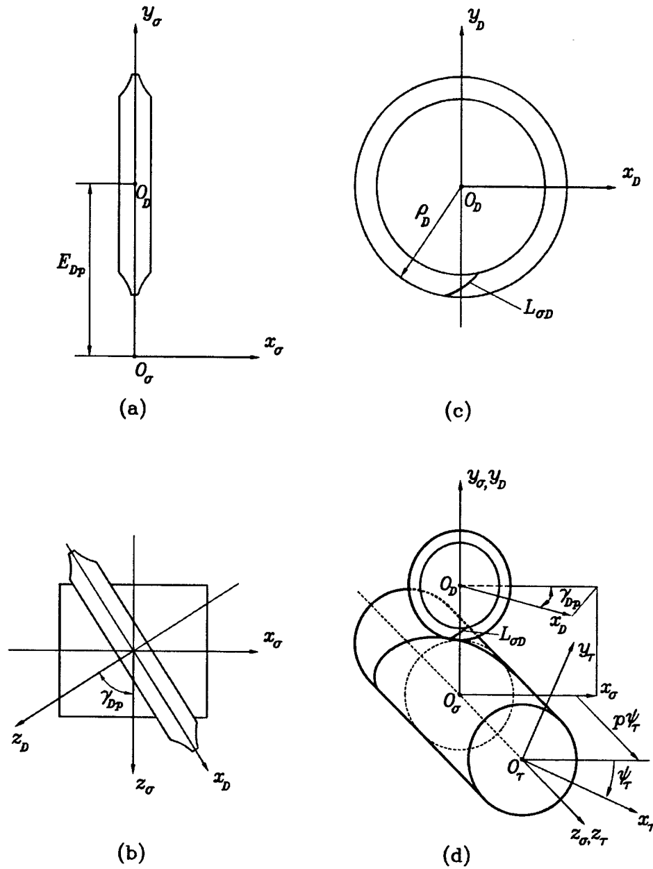
Figure 18.—Determination of disk surface \Sigma_D . (a) and (b) Installment of grinding disk. (c) Line L_{\sigma D} of tangency of surfaces \Sigma_{\sigma} and \Sigma_D . (d) Illustration of generation of surface \Sigma_{\tau} by disk surface \Sigma_D .
