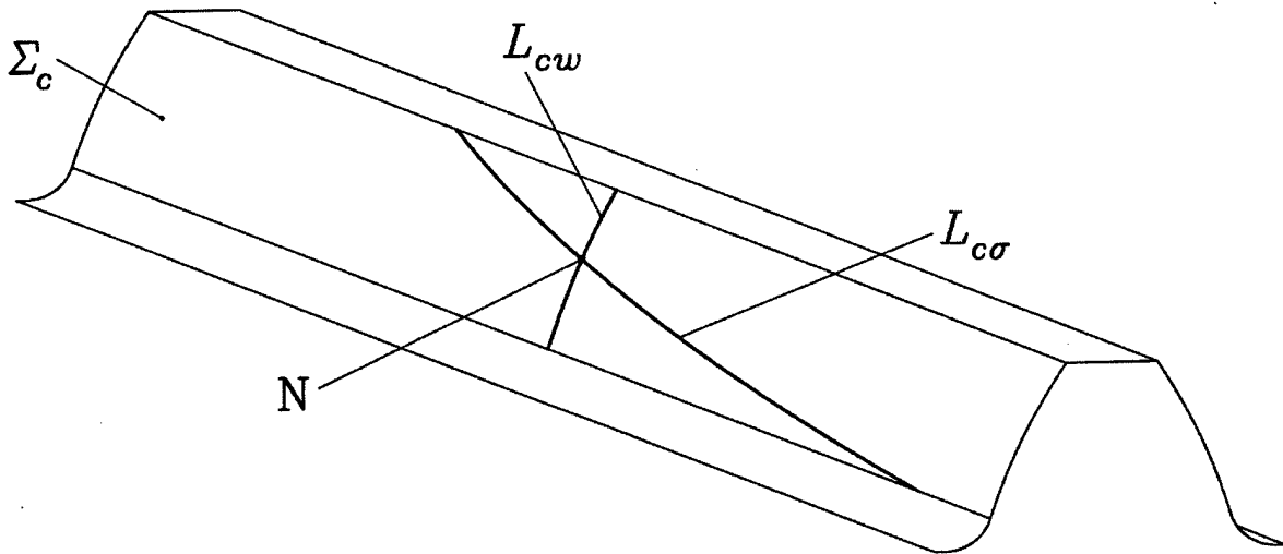
Figure 23.—Contact lines L_{c\sigma} and L_{c\omega} corresponding to meshing of rack-cutter \Sigma_c with pinion and worm surfaces \Sigma_p and \Sigma_w , respectively.
