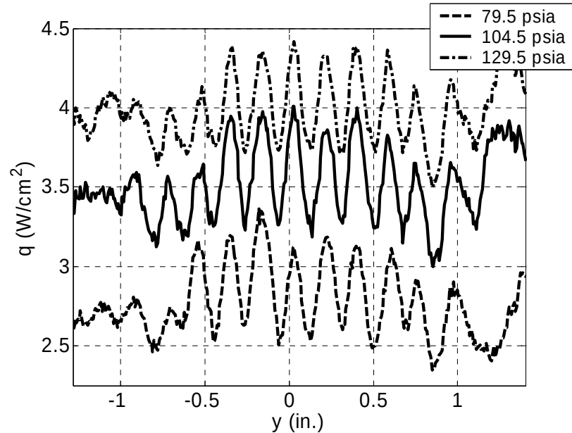
Figure 8.13. Comparison of the spanwise heat-transfer-rate distribution on the 2 nd compression ramp against the initial total pressure.
