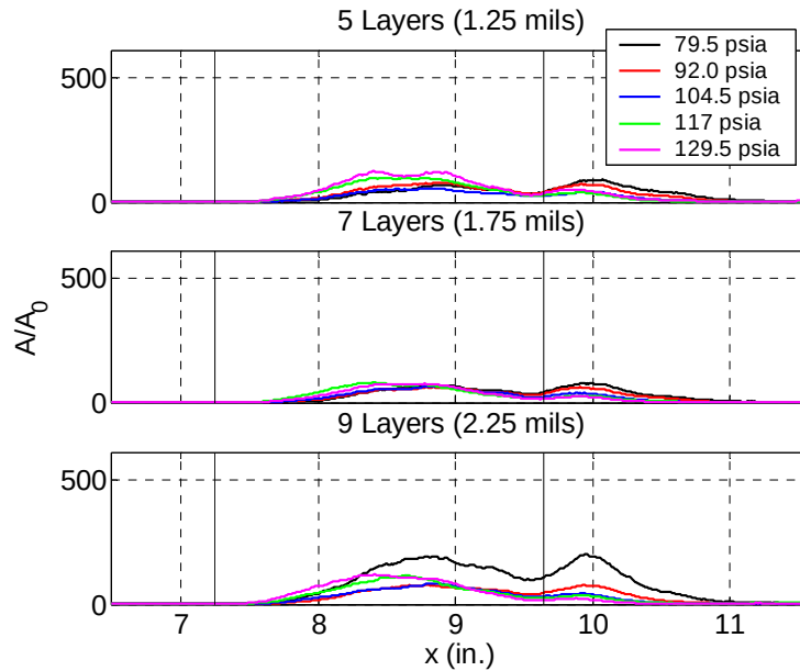
Figure 8.33. Streamwise growth of the amplitude ratio. All cases shown are for the cases with 21 roughness strips (0.125 inch spacing).
