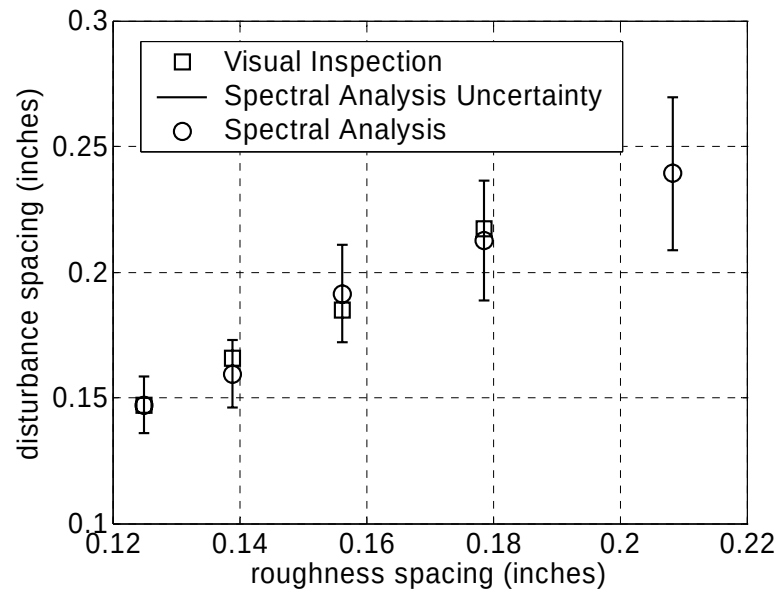
Figure 8.19. Spacing of the streamwise vortices against the roughness spacing.
