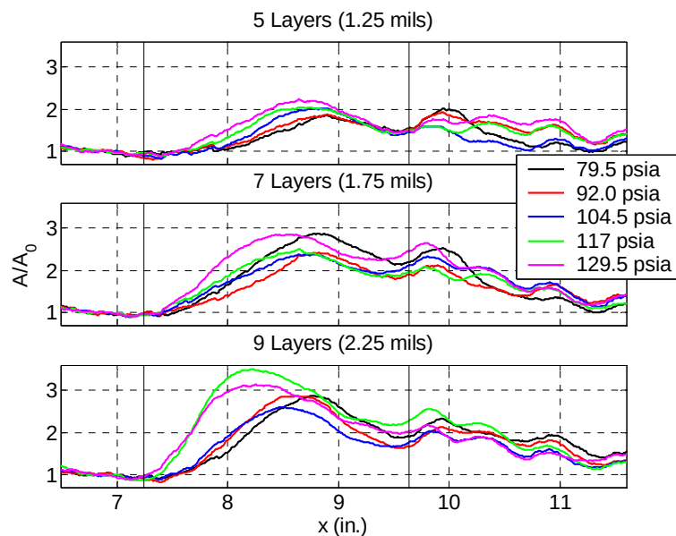
Figure 8.23. Streamwise growth of the RMS heat-transfer-rate fluctuation amplitude ratios. All cases shown are for the cases with 15 roughness strips (0.18 inch spacing).
