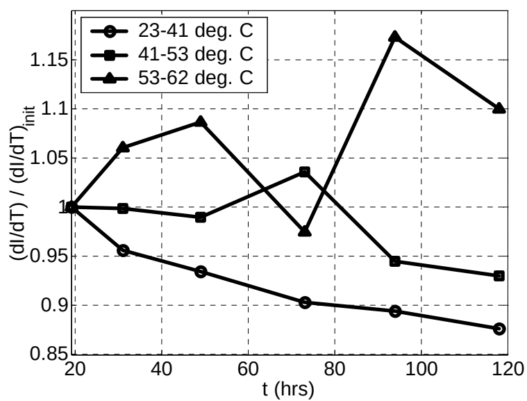
Figure 3.8. Variation of the temperature sensitivity at three temperatures.
