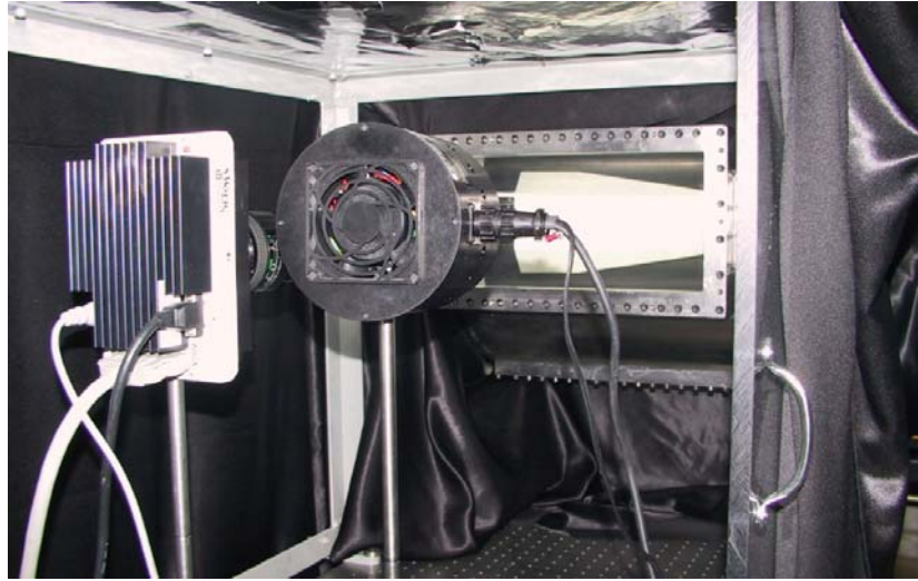
Figure 4.2. Image of the experimental setup.
