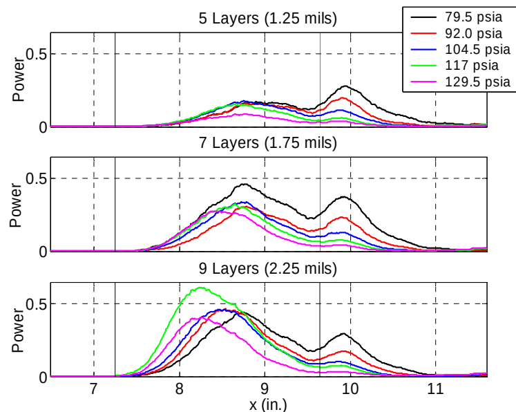
Figure 8.28. Streamwise growth of the power. All cases shown are for the cases with 15 roughness strips (0.18 inch spacing).
