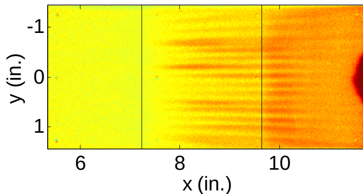
Figure 6.8. Heat transfer rate distribution on the Hyper-2000 near the compression corners.
