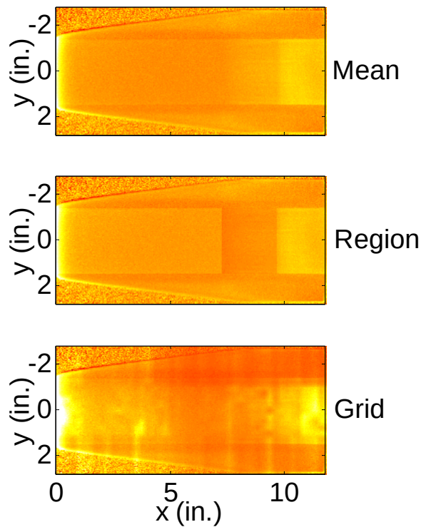
Figure 6.3. Heat transfer rate distributions computed with three different treatment of the insulator thickness distributions.
