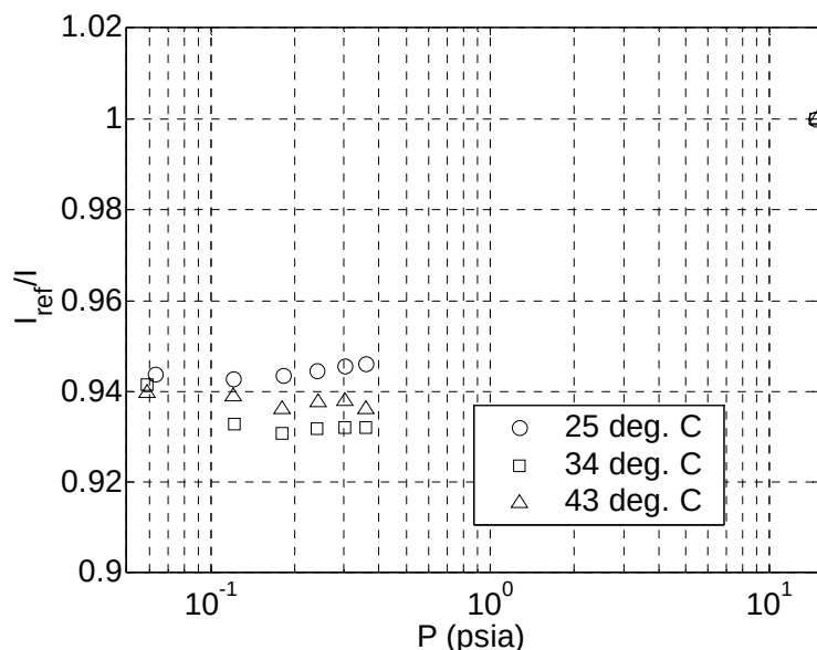
Figure 3.5. Sensitivity of the TSP to pressure variation at three temperature values.
