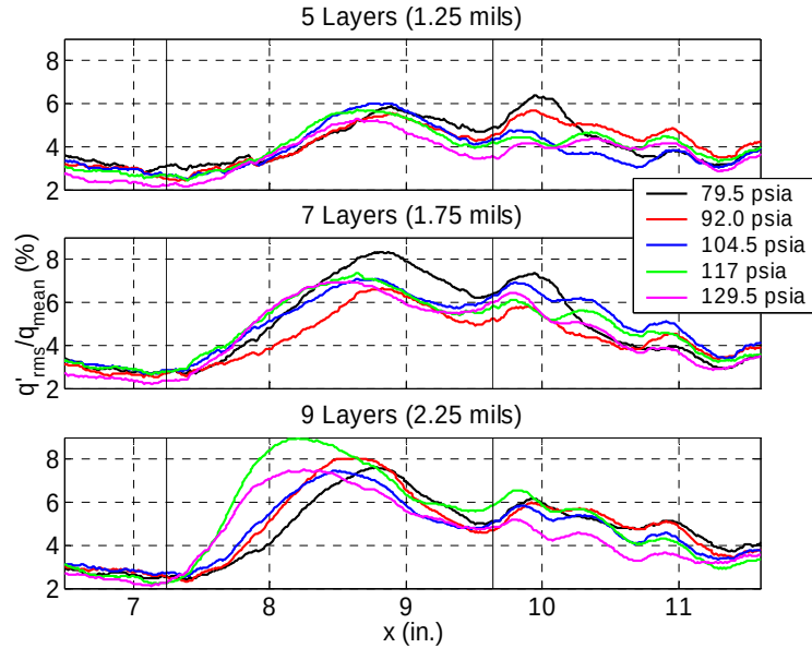
Figure 8.22. Streamwise growth of the RMS heat-transfer-rate fluctuations. All cases shown are for the cases with 15 roughness strips (0.18 inch spacing).
