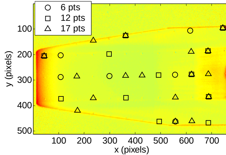
Figure 5.5. Optimized registration mark locations for the 2 nd order polynomial image registration equation.
