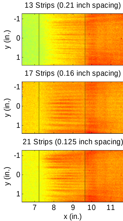
Figure 8.10. Effect of leading edge roughness spacing. The cases shown used three layers (2.25 mils) of roughness strips, all at a total pressure of 129.5 psia (2.72 million/ft).
