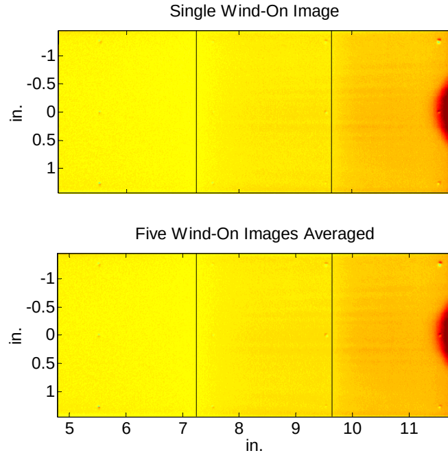
Figure 4.4. Uncalibrated temperature image obtained using a single wind-off image, and using the average of five wind-off images.
