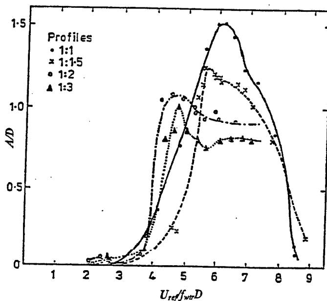
Fig. 28. The maximum A/D for the no-shear case (about 1.5 at U_{ref}/f_{wtr}D = 6.2 ) corresponds quite well with that in Fig. 26 (about 1.5 at U_{ref}/f_{wtr}D = 7 ). With shear, the maximums of A/D occur with reduced peaks at smaller U_{ref}/f_{wtr}D and decrease towards unity. It appears that shear extends the range of the lock-in region. Even in the critical Re region, the occurrence of maximum C_d (at about U_{ref}/f_{wtr}D = 5.6 ) precedes the occurrence of maximum A/D (at U_{ref}/f_{wtr}D \approx 6.2 ), as in Figs. 26(a) and (b) for the sub-critical flow (Humphries and Walker, 1988).
