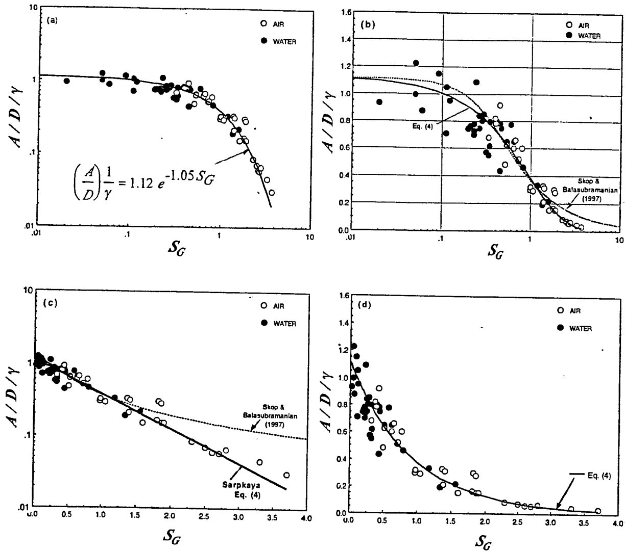
Fig. 7 Experimental measurements of the modally normalized maximum amplitude versus the response parameter S_G and the proposed curve-fit (Eq. (4)). The data is tabulated in Skop & Balasubramanian (1997): ●, water; ○, air. The above figures show: (a) a Log-Log plot, (b) a linear-Log plot, (c) a Log-linear plot, and (d) a linear-linear plot. In each case Eq. (4) represents the data reasonably well and makes an unrigorous but plausible suggestion that \ln(A/D/\gamma) may be a linear function of S_G .
