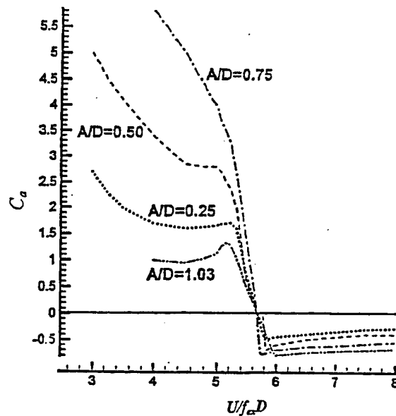
Fig. 25. Variation of the inertia coefficient C_a (in-phase component of the transverse force) with V_r = U/f_a D for representative values of A/D (from Sarpkaya 1978, V_r is multiplied by 1.13 to match the Strouhal numbers at critical transitions).
