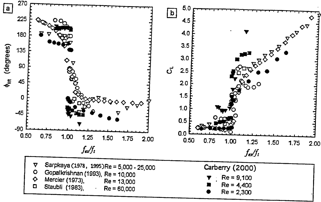
Fig. 11. (a) and (b) show the phase angle ( \phi_{lift} ) and the lift coefficient C_L in terms of f_\alpha/f_i . Apparently, the data for Re less than about 10^4 – 1.5 \times 10^4 differ most from the rest even in a plot pulled together by f_\alpha/f_i . This suggests that the average position of the transition from a disturbed-laminar state to a turbulent state in the free shear layers has not yet fully migrated upstream. (from Carberry, 2000).
