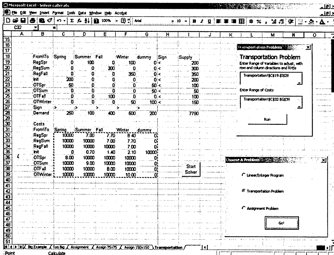
Figure 5: Transportation Problem. The user supplies signs and values for each row and column constraint (upper matrix). The costs (lower matrix) include shaded cells set to a large value as a penalty. The optimal value of 7790 is visible in the bottom right-hand corner of the constraint matrix.
