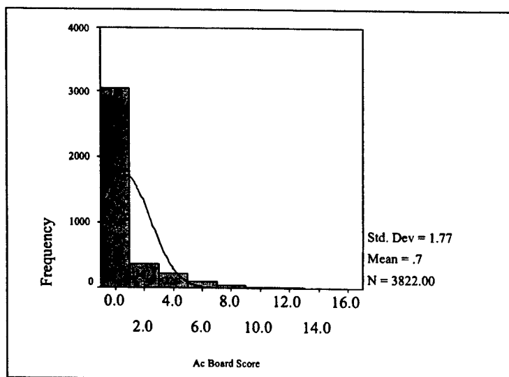
Figure 5. Frequency Distribution of ACBDSCR with Normal Curve
