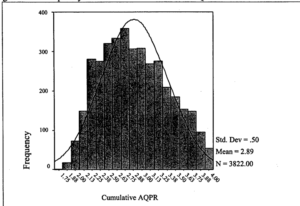
Figure 4. Frequency Distribution of Cumulative AQPR with Normal Curve
