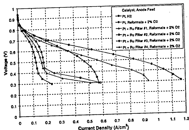
Figure 9. Single-cell performance comparison of the Pt + Ru filter for an anode feed of reformate + 2% \text{O}_2 . P = 1 \text{ atm} , T = 70^\circ\text{C} . The filter configurations are defined as follows: filter no. 1 ( \blacktriangle ) contains 35 wt % Nafion and is placed on the membrane side of the GDL; filter no. 2 ( \circ ) contains 35 wt % Nafion and is placed on the flowfield side of the GDL; filter no. 3 ( \square ) contains 10 wt % Nafion and is placed on the membrane side of the GDL; filter no. 4 ( \triangle ) contains 10 wt % Nafion and is placed on the flowfield side of the GDL.
