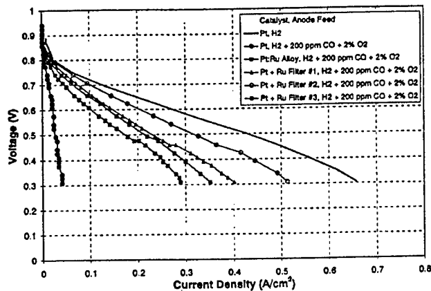
Figure 5. Performance comparison of MEUs with sputter-deposited Ru filter for an anode feed of hydrogen + 200 ppm CO + 2% O_2 . P = 1 atm, T = 70^\circ C . The filter configurations are defined in Fig. 3.
