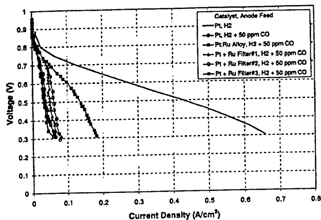
Figure 3. Performance comparison of MEUs with sputter-deposited Ru filter under H_2 + 50 ppm CO conditions. P = 1 atm, T = 70^\circ C . The filter configurations are defined as follows: filter 1 ( \blacktriangle ) is the standard Ru filter prepared from an ink; filter 2 ( \circ ) is a single 25 min sputter-deposited layer of Ru separated from the Pt electrode by a layer of NCI; filter 3 ( \square ) is a three-layer sputter-deposited Ru filter (8.33 min per layer, see Fig. 2 for design) separated from the Pt electrode by a layer of NCI.
