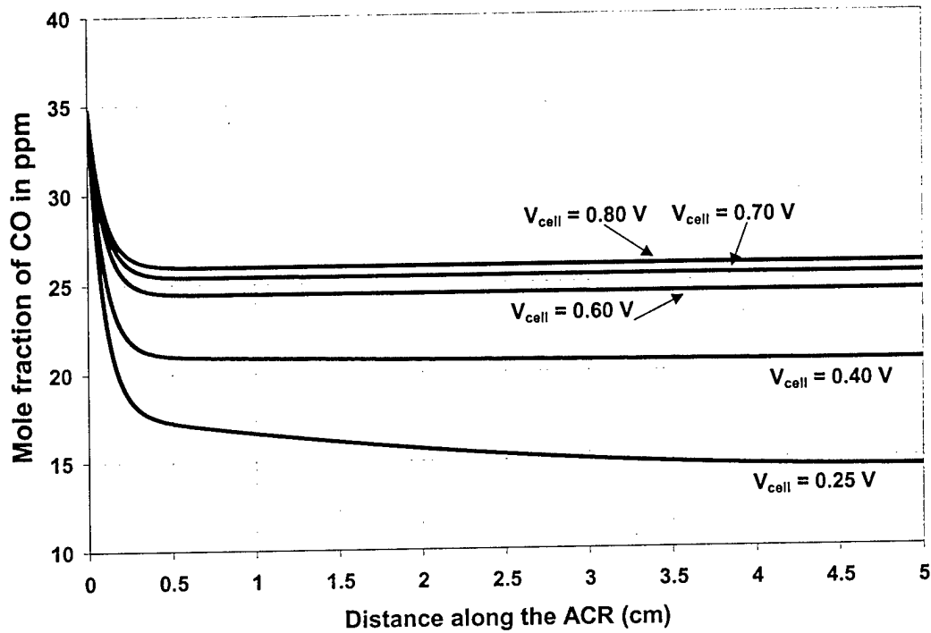
Figure 12 The calculation of CO concentration along the length of the anode catalyst region for a fully humidified anode stream. P = 1 \text{ atm} , T = 70^\circ\text{C} . Initial feedstream composition (dry): x_{\text{H}_2} = 0.40 , x_{\text{CO}} = 50 \text{ ppm} , and 1% \text{O}_2 (relative to \text{H}_2 ). b_{\text{O}_2} = 0.48 \text{ V} , k_{f\text{O}_2} = 7 \times 10^{-4} \text{ A cm}^{-2} \text{ atm}^{-1} and k_{e\text{O}_2} = 3 \times 10^{-3} \text{ A cm}^{-2} \text{ atm}^{-1} .
