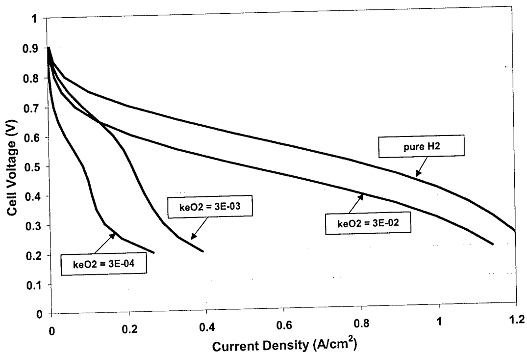
Figure 16 The effect of varying the rate constant, k_{eO_2} , for the electrochemical oxidation of CO by O_2 on PEMFC performance. P = 1\text{atm} , T = 70^\circ\text{C} . Initial feedstream composition (dry): x_{H_2} = 0.40 , x_{CO} = 50\text{ ppm} , and 1% O_2 (relative to H_2 ). b_{O_2} = 0.48\text{ V} , k_{fO_2} = 7 \times 10^{-4}\text{ A cm}^{-2}\text{ atm}^{-1} .
