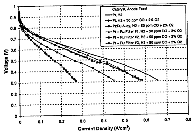
Figure 4. Performance comparison of MEUs with sputter-deposited Ru filter for an anode feed of hydrogen + 50 ppm CO + 2% O_2 . P = 1 atm, T = 70^\circ C . The filter configurations are defined in Fig. 3.
