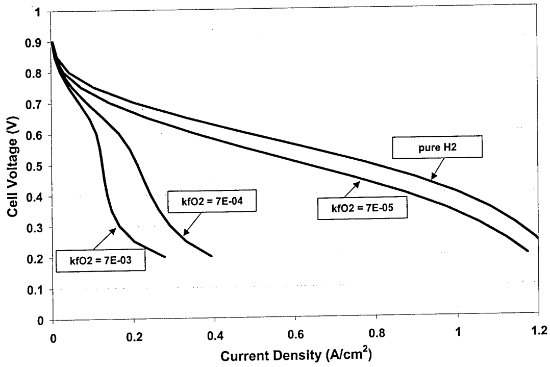
Figure 14 The effect of varying the rate constant, k_{fO_2} , for the catalytic reaction between H_2 and O_2 on PEMFC performance. P = 1\text{atm} , T = 70^\circ\text{C} . Initial feedstream composition (dry): x_{H_2} = 0.40 , x_{CO} = 50\text{ ppm} , and 1\% O_2 (relative to H_2 ). b_{O_2} = 0.48\text{ V} , k_{eO_2} = 3 \times 10^{-3}\text{ A cm}^{-2}\text{ atm}^{-1} .
