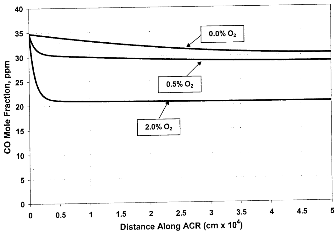
Figure 6 The calculation of CO concentration along the length of the anode catalyst region for various O 2 concentrations. P = 1atm, T = 70°C, V CELL = 0.4 V.
