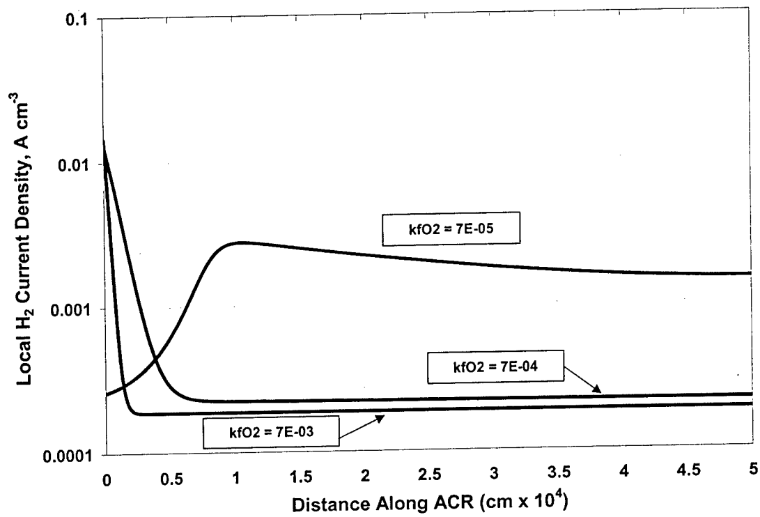
Figure 15 The effect of varying the rate constant, k_{fO_2} , for the catalytic reaction between H 2 and O 2 on local hydrogen current density, j_h , along the length of the ACR. P = 1\text{atm} , T = 70^\circ\text{C} . Initial feedstream composition (dry): x_{H_2} = 0.40 , x_{CO} = 50\text{ ppm} , and 1% O 2 (relative to H 2 ). b_{O_2} = 0.48\text{ V} , k_{eO_2} = 3 \times 10^{-3}\text{ A cm}^{-2}\text{ atm}^{-1} .
