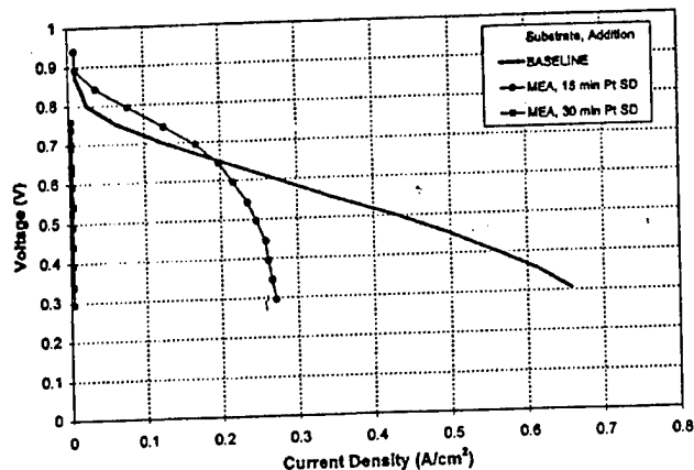
Figure 5. Performance comparison of baseline MEAs onto which various amounts of Pt has been sputter deposited. P = 1 \text{ atm} , T = 70^\circ\text{C} .
