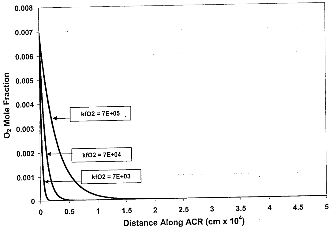
Figure 17 The effect of varying the rate constant, k_{fO_2} , for the catalytic reaction between H_2 and O_2 on oxygen concentration, x_{O_2} , along the length of the ACR. P = 1\text{atm} , T = 70^\circ\text{C} . Initial feedstream composition (dry): x_{H_2} = 0.40 , x_{CO} = 50\text{ ppm} , and 1% O_2 (relative to H_2 ). b_{O_2} = 0.48\text{ V} , k_{eO_2} = 3 \times 10^3\text{ A cm}^{-2}\text{ atm}^{-1} .
