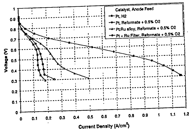
Figure 5. Single-cell performance comparison of Pt, Pt:Ru, and Pt + Ru filter for an anode feed of reformate + 0.5% O 2 bleed. P = 1 atm, T = 70^\circ\text{C} .
