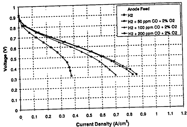
Figure 8. Single-cell performance comparison of the Pt + Ru filter for an anode feed consisting of hydrogen + 2% \text{O}_2 + various CO concentrations. P = 1 \text{ atm} , T = 70^\circ\text{C} .
