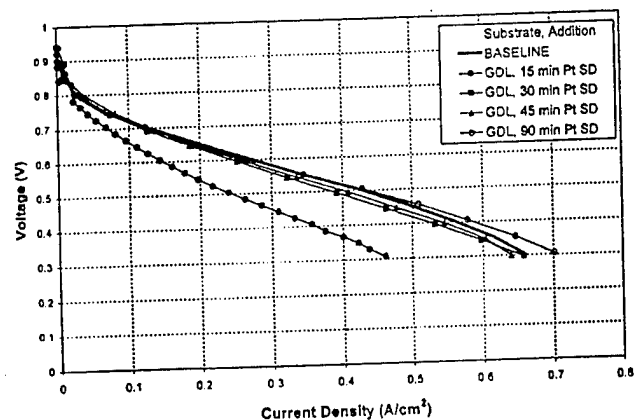
Figure 4. Performance comparison for MEUs prepared from GDLs with various sputter-deposited Pt loadings. P = 1 \text{ atm} , T = 70^\circ\text{C} .
