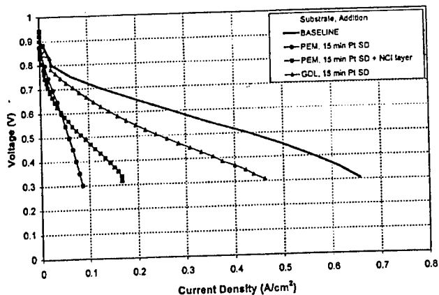
Figure 6. Performance comparison of MEUs prepared from PEMs and GDLs with one or several layers of sputter-deposited Pt. P = 1 \text{ atm} , T = 70^\circ\text{C} .
