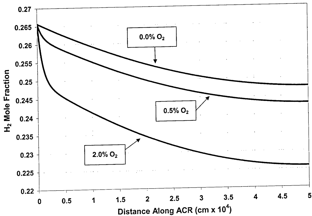
Figure 9 The calculation of H 2 concentration along the length of the anode catalyst region when CO and O 2 are added to the feedstream. P = 1atm, T = 70°C, V CELL = 0.4 V.
