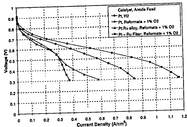
Figure 4. Single-cell performance comparison of Pt, Pt:Ru, and Pt + Ru filter for an anode feed of reformate + 1% O 2 bleed. P = 1 atm, T = 70^\circ\text{C} .
