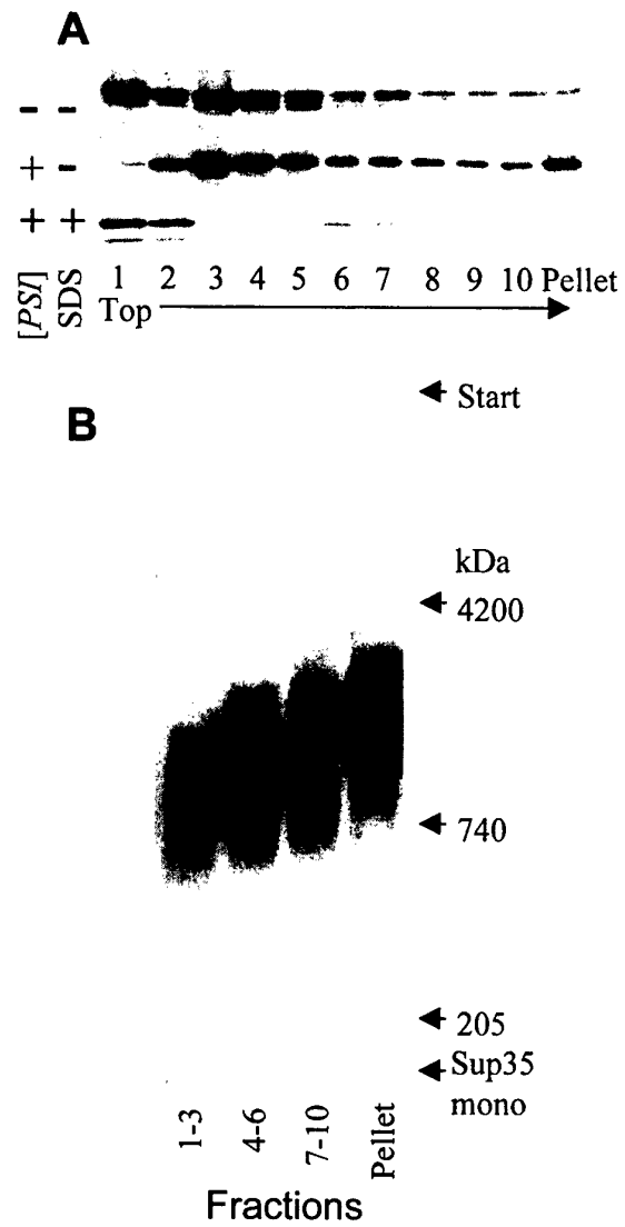
Figure 5. SDS disassembles Sup35 prion aggregates into smaller SDS-resistant particles.
