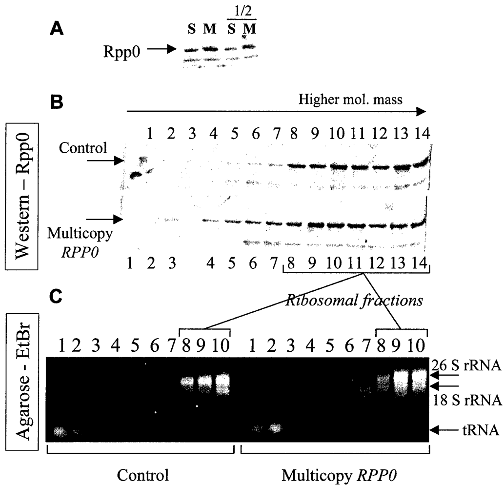
Figure 2. Overproduced Rpp0 accumulates in sub-ribosomal fractions. Lysates were prepared from the PS-5V-H19 [ psi r ] transformants with either the Yeplac195 vector (C, control) or multicopy RPP0 plasmid (M, m RPP0 ) (A) Comparison of the Rpp0 levels by Western blotting of total lysates; S, 50% load. (B) The lysates were fractionated by centrifugation and analyzed for Rpp0 by Western blotting. The Rpp0 levels are increased compared to control in sub-ribosomal fractions 3 to 7. (C) Determination of the fractions containing ribosomes. The same fractions were separated on agarose gel and stained with Ethidium Bromide. The 26S and 18S ribosomal RNAs are present in fractions 8 and higher.
